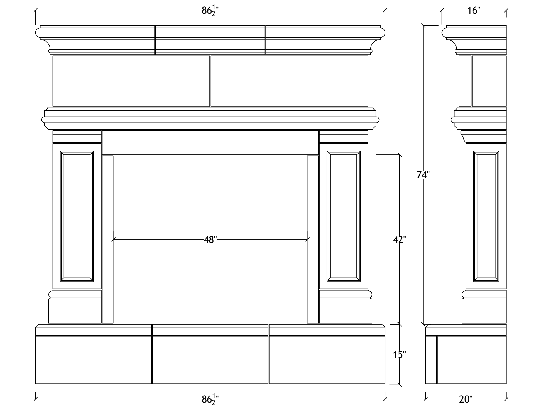
48" Windsor with raised hearth
