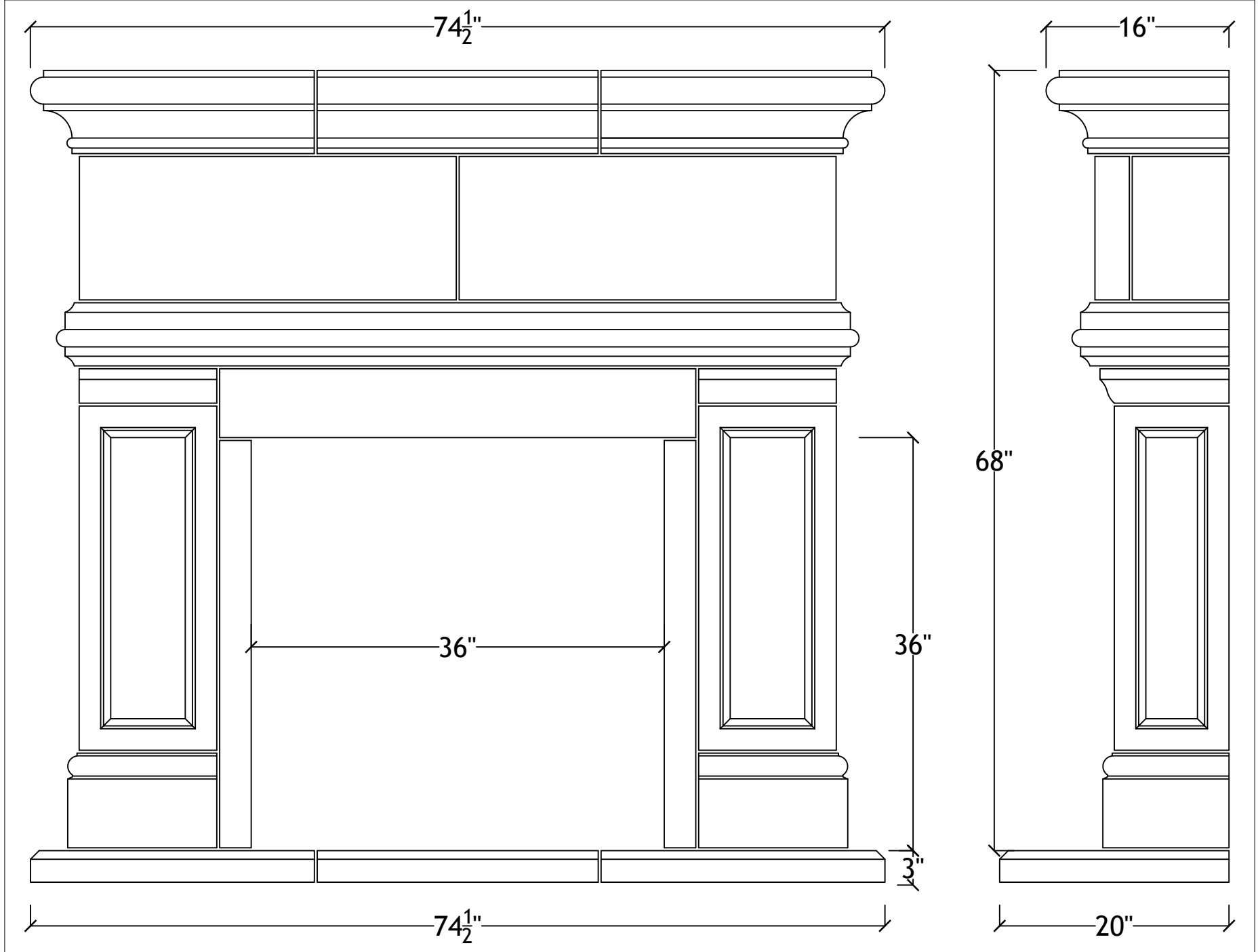
36" Windsor with hearth
