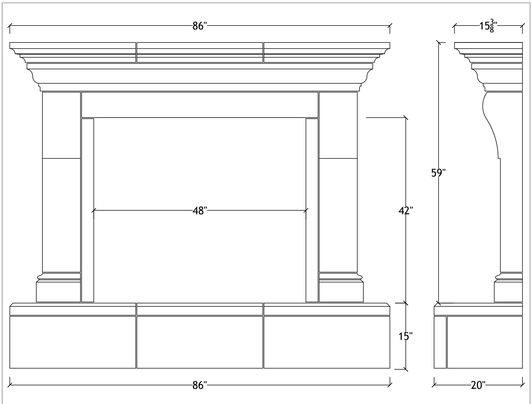
48" Whitmoore with raised hearth
