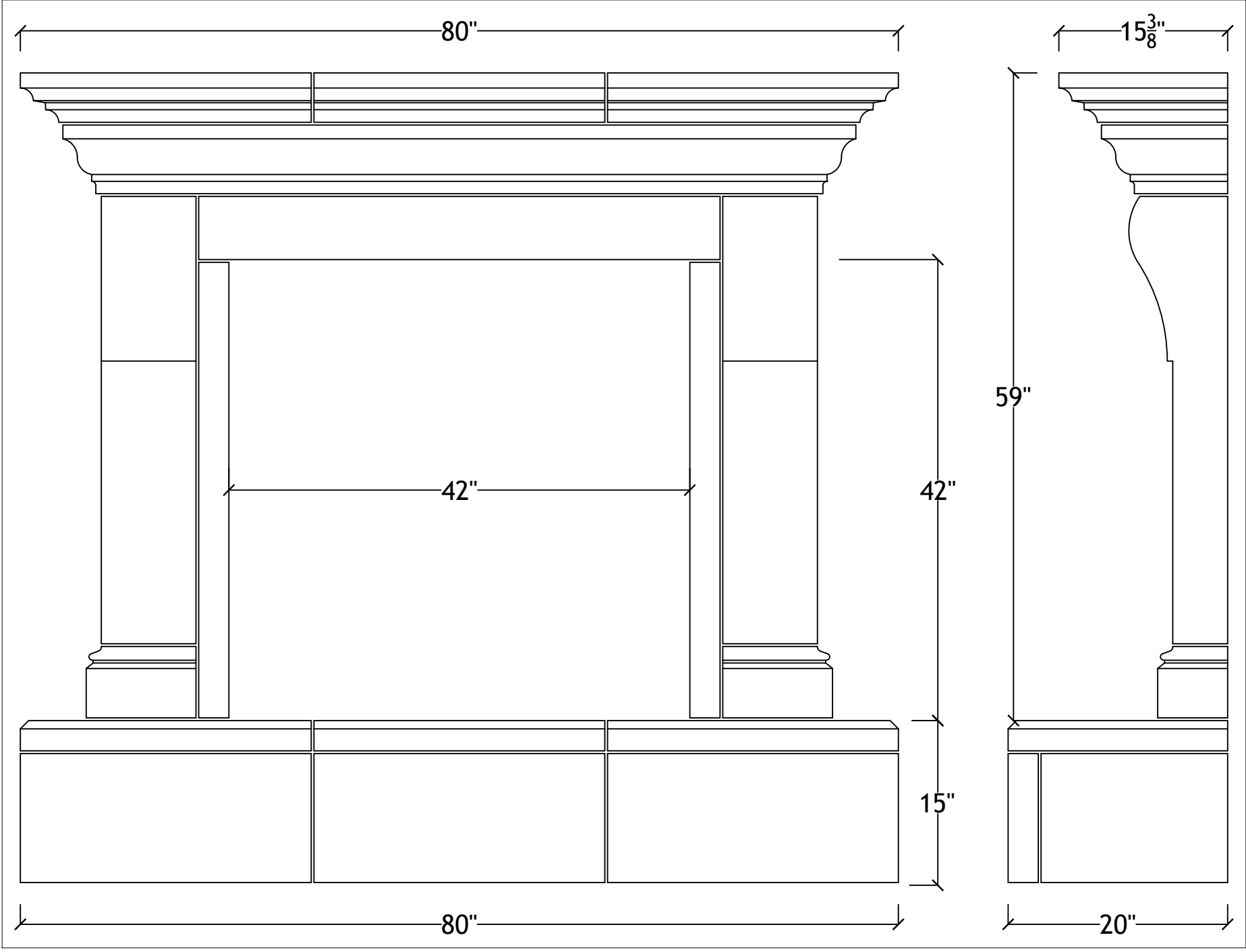
42" Whitmoore with raised hearth
