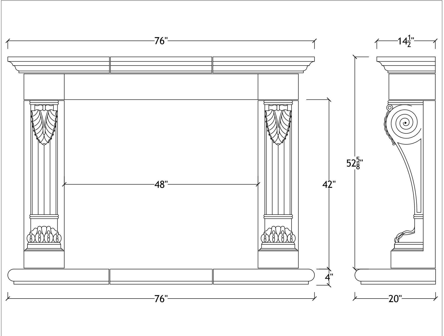
48" Wellington with bullnosed hearth
