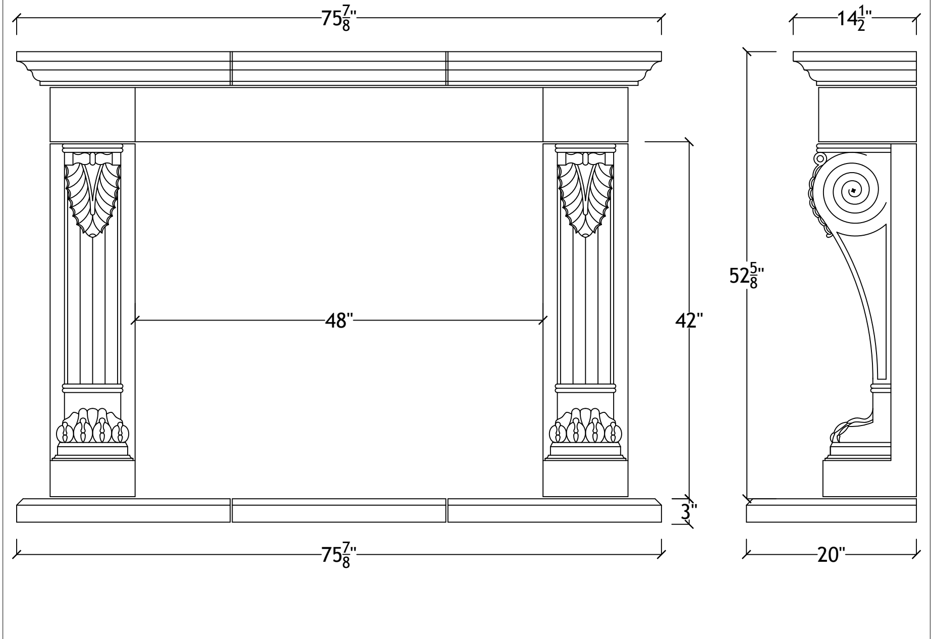
48" Wellington with hearth
