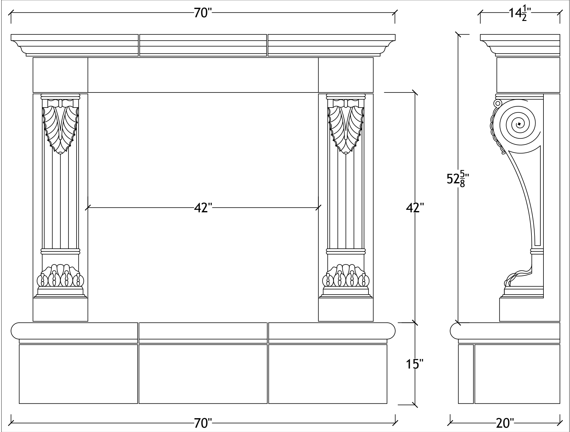
42" Wellington with raised bullnosed hearth
