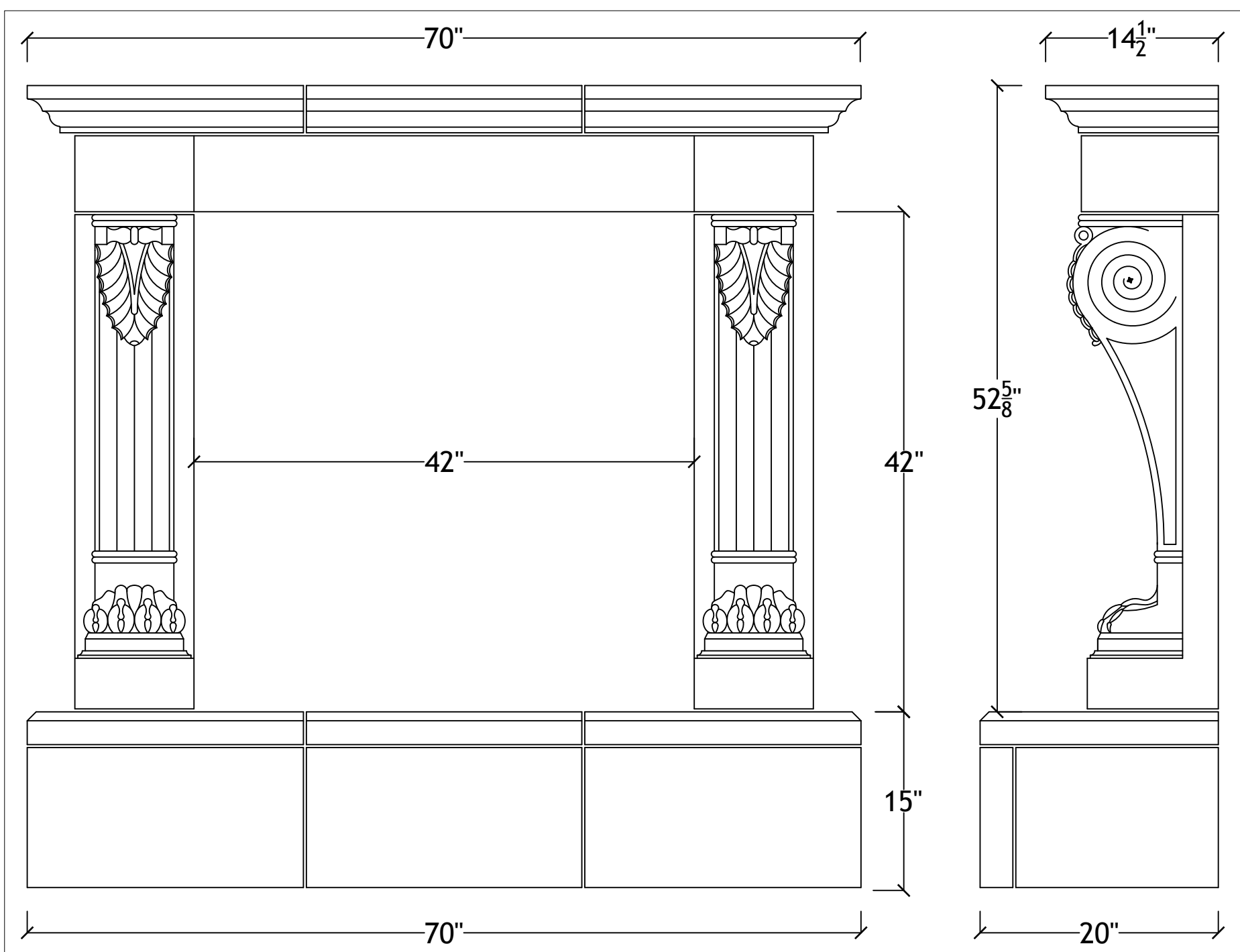
42" Wellington with raised hearth
