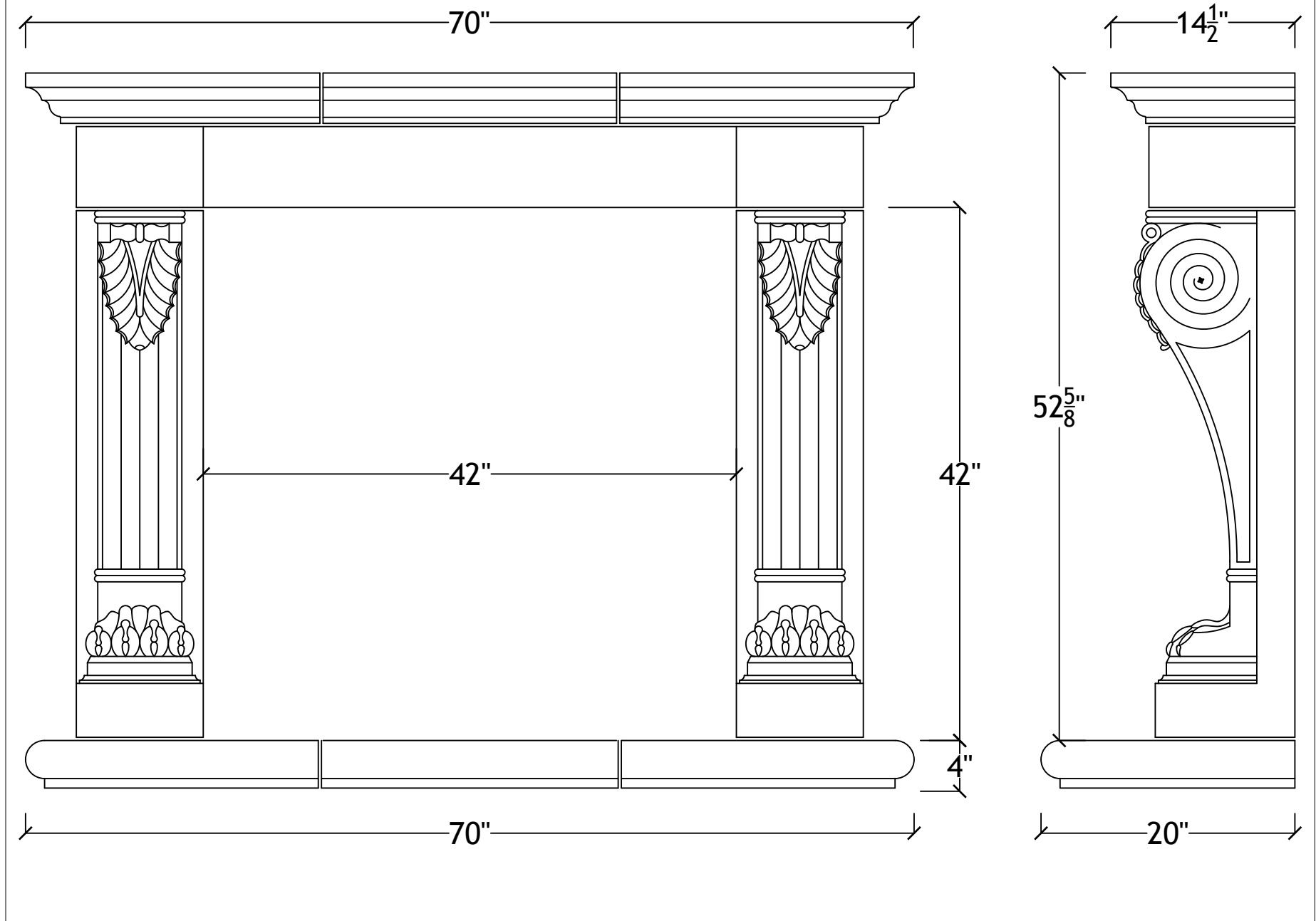
42" Wellington with bullnosed hearth
