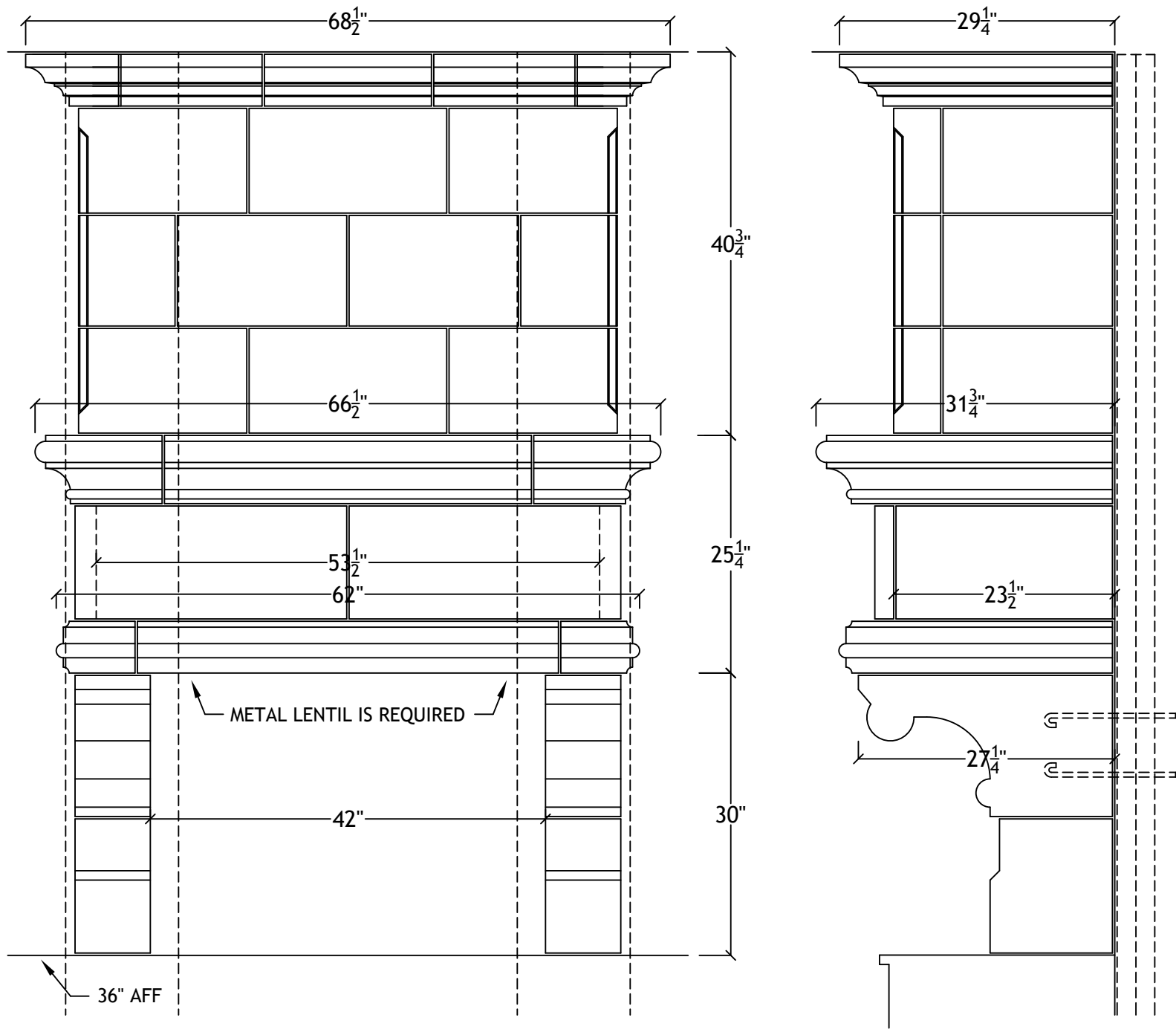
42" Waverly Range Hood for 11' ceiling
