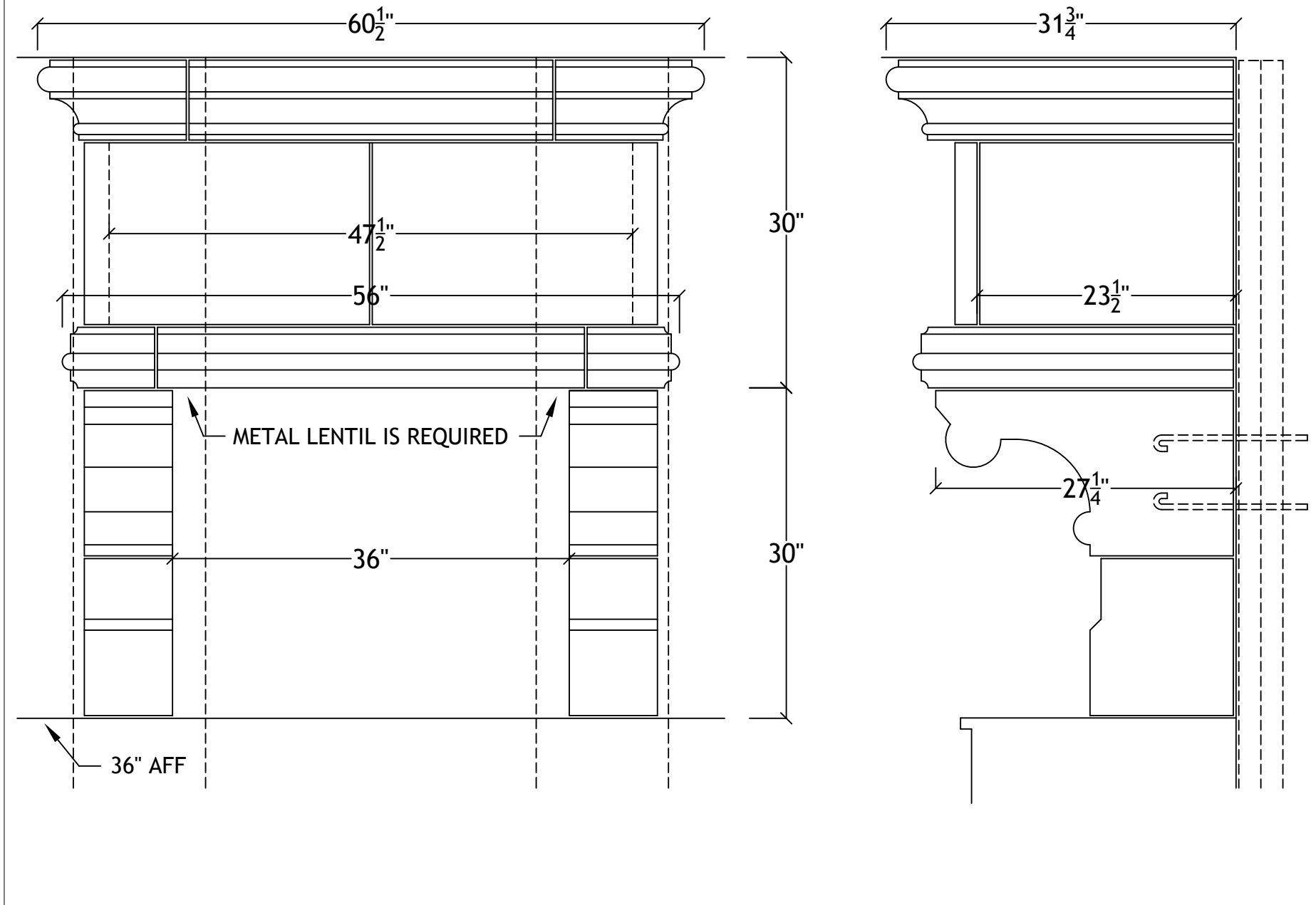
36" Waverly Range Hood for 8' ceiling
