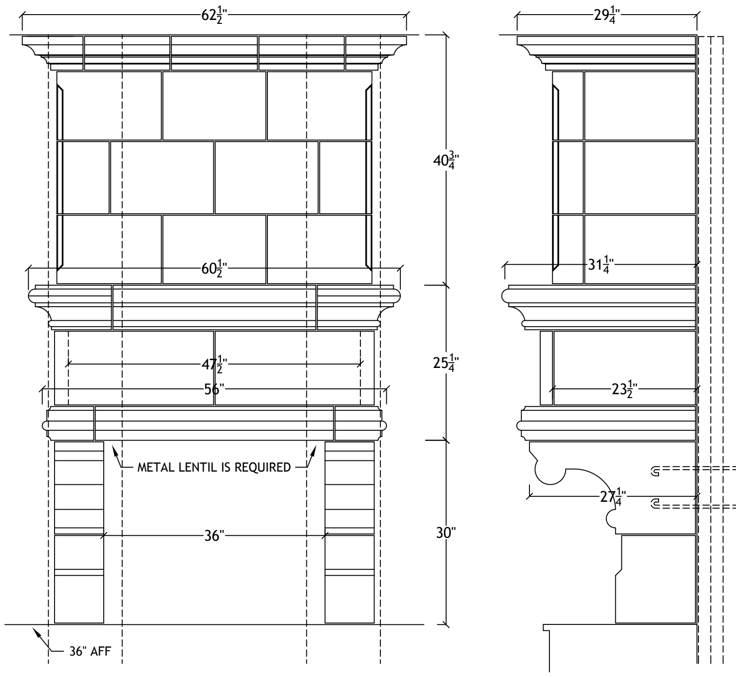
36" Waverly Range Hood for 11' ceiling
