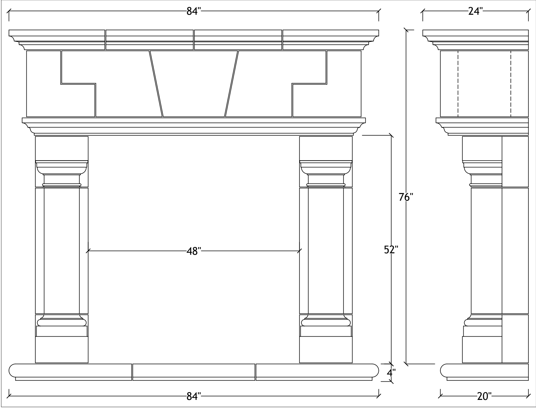
48" Valencia with bullnosed hearth
