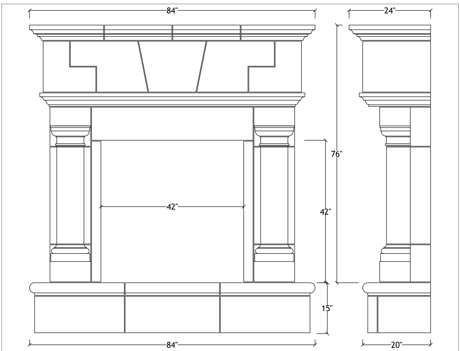
42" Valencia with raised bullnosed hearth
