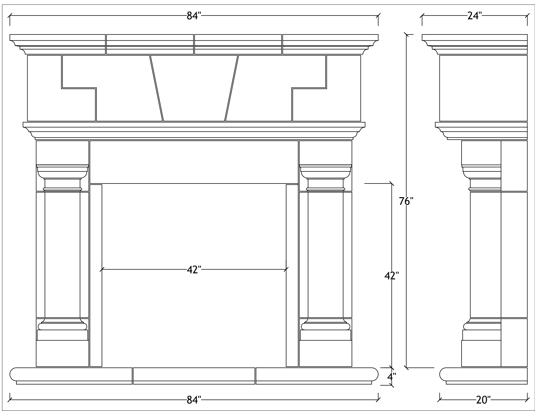
42" Valencia with bullnosed hearth
