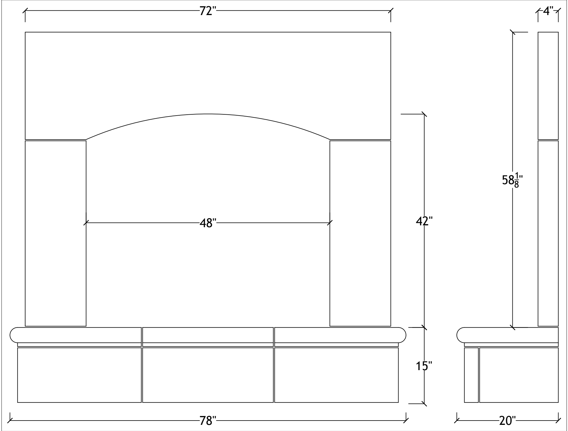
48" Urban with raised bullnosed hearth
