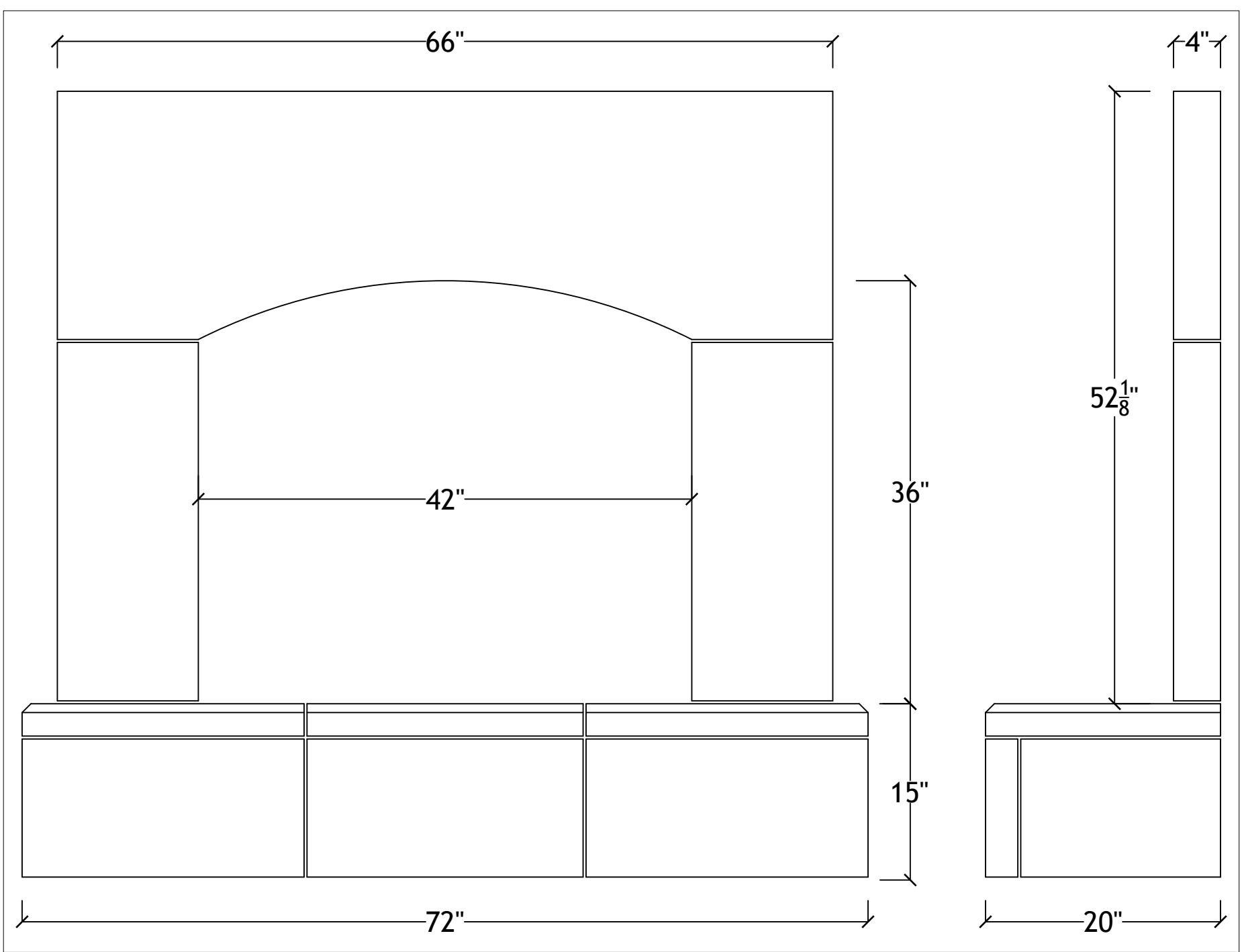
42" Urban with raised hearth
