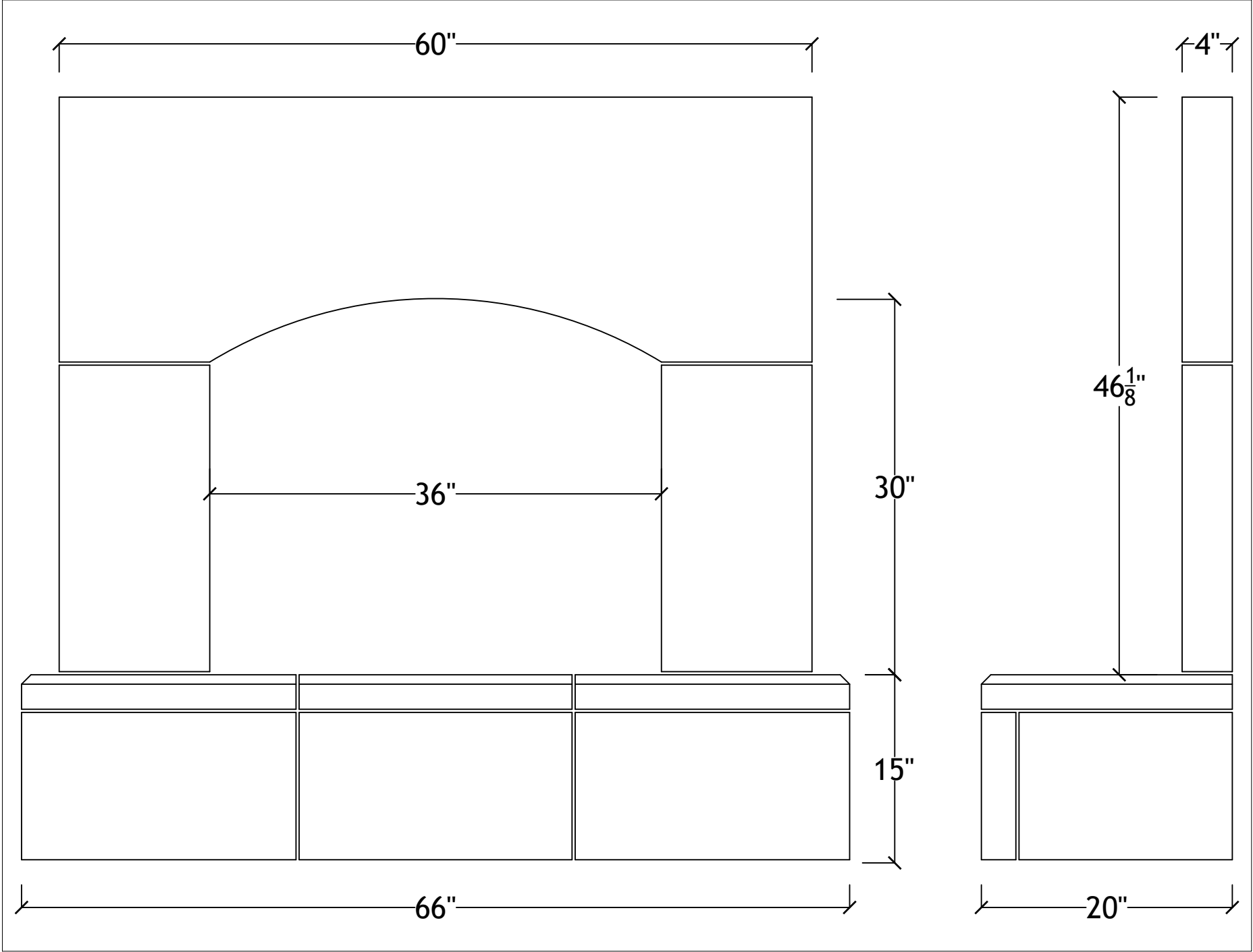
36" Urban with raised hearth
