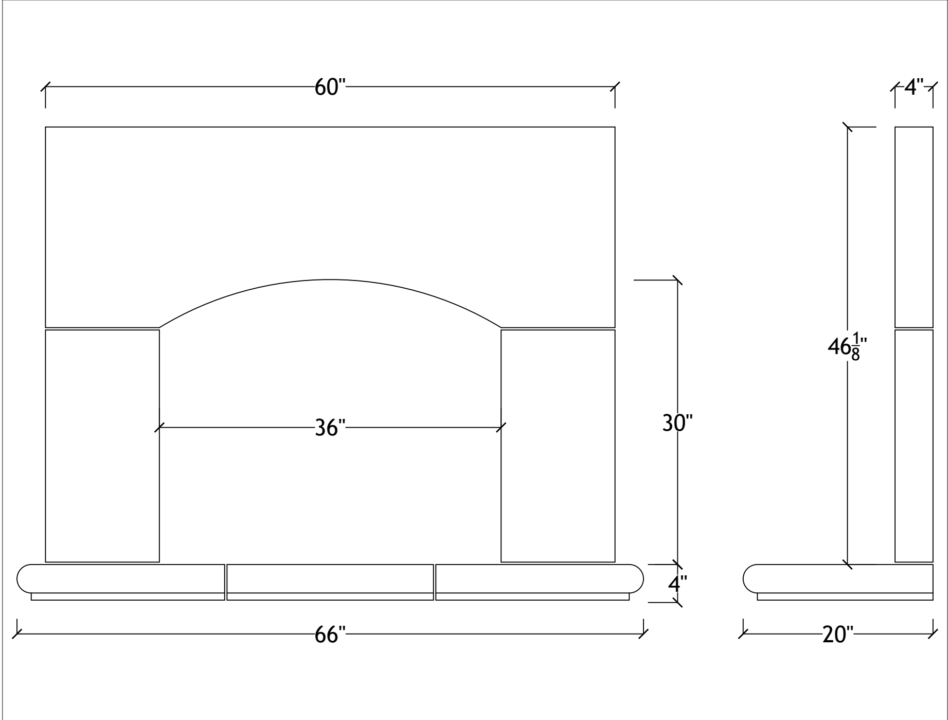
36" Urban with bullnosed hearth
