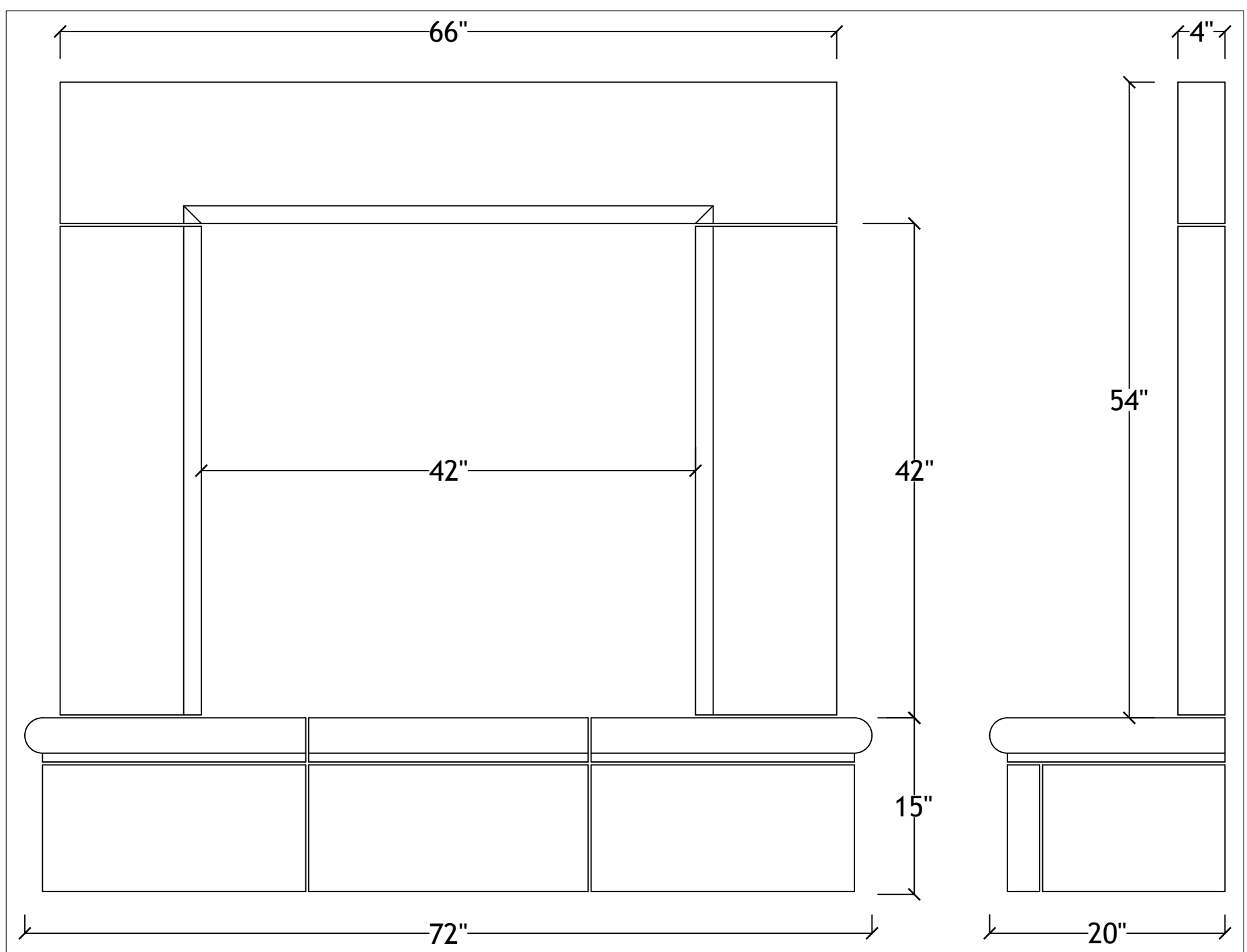
42" Uptown with raised bullnosed hearth
