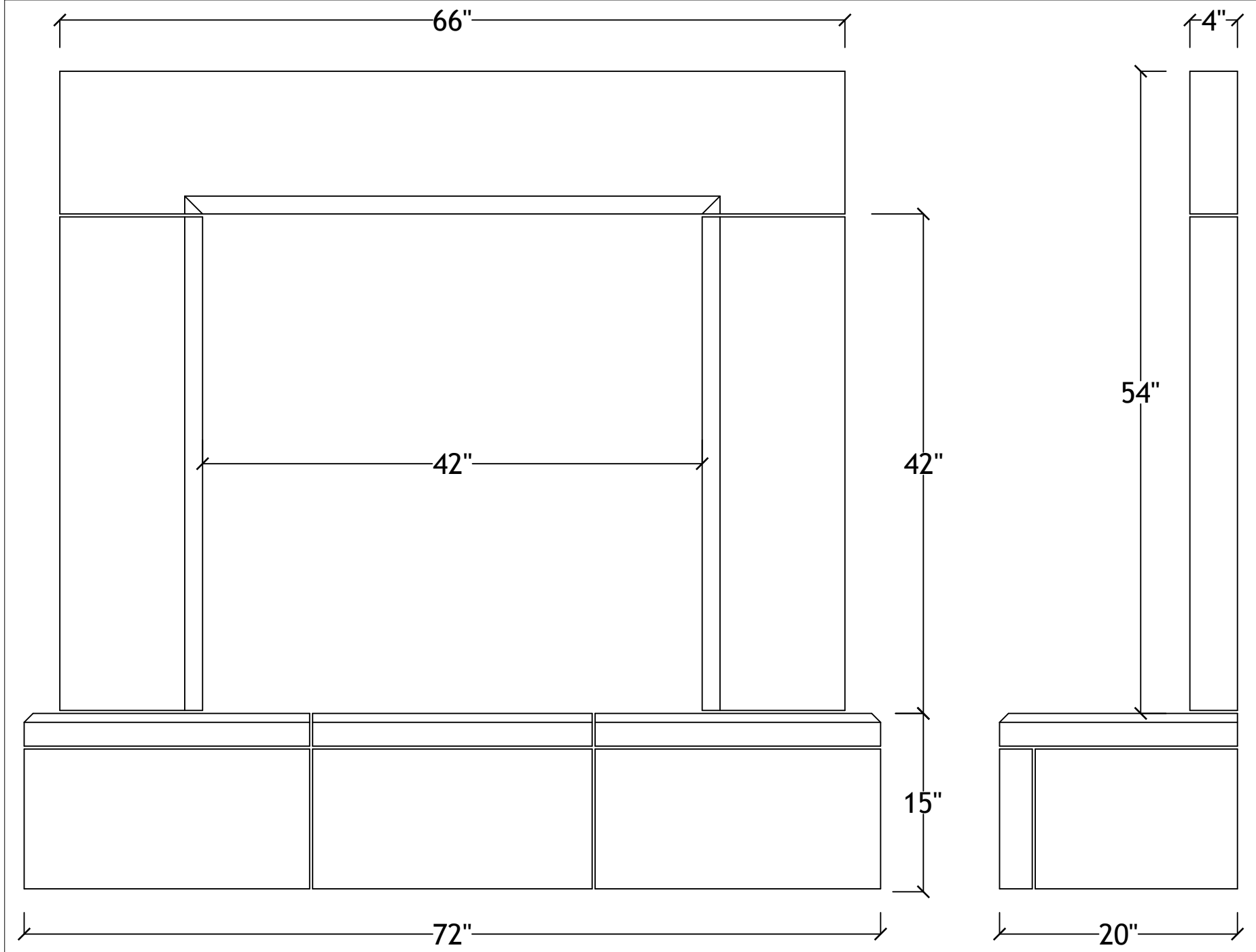
42" Uptown with raised hearth
