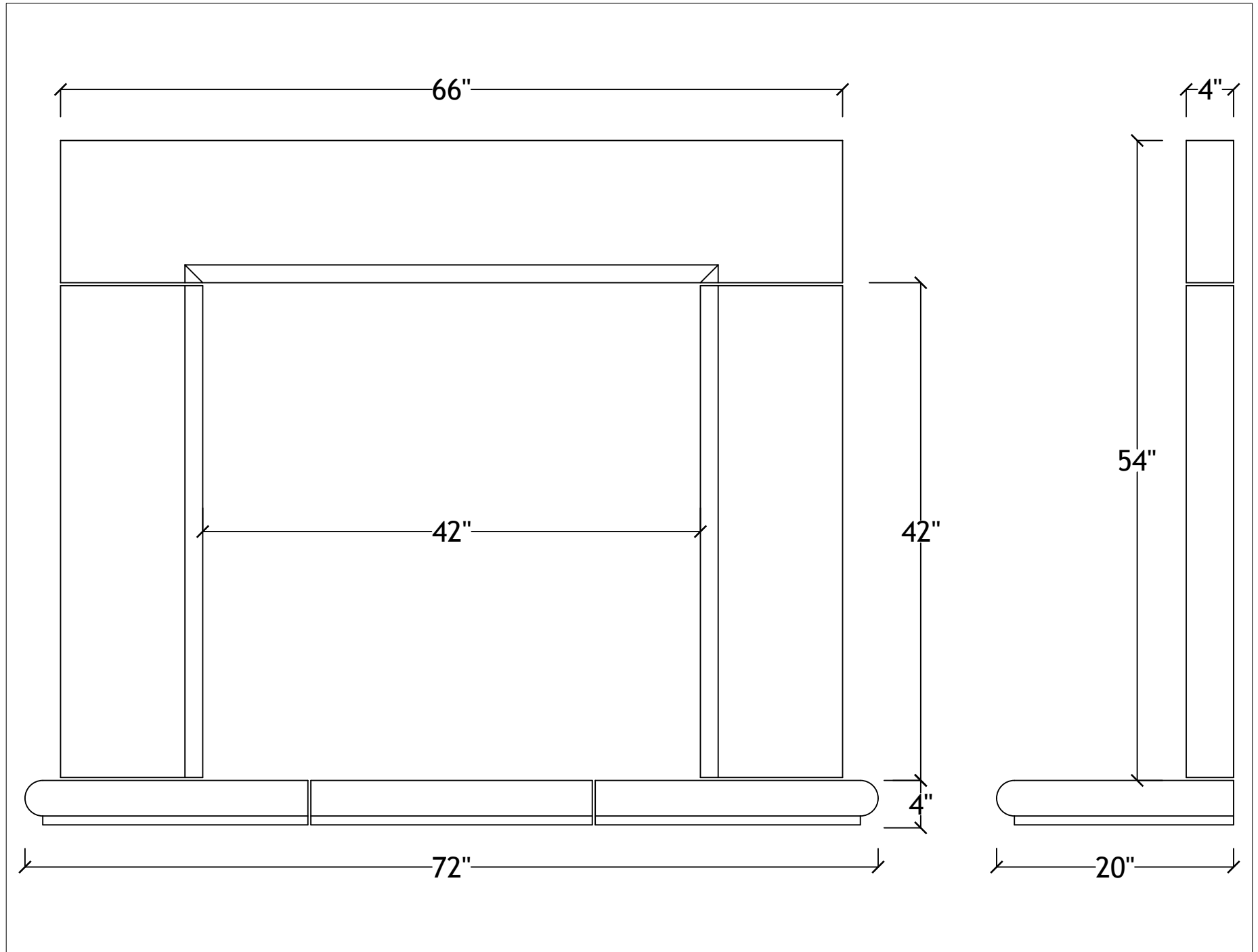
42" Uptown with bullnosed hearth
