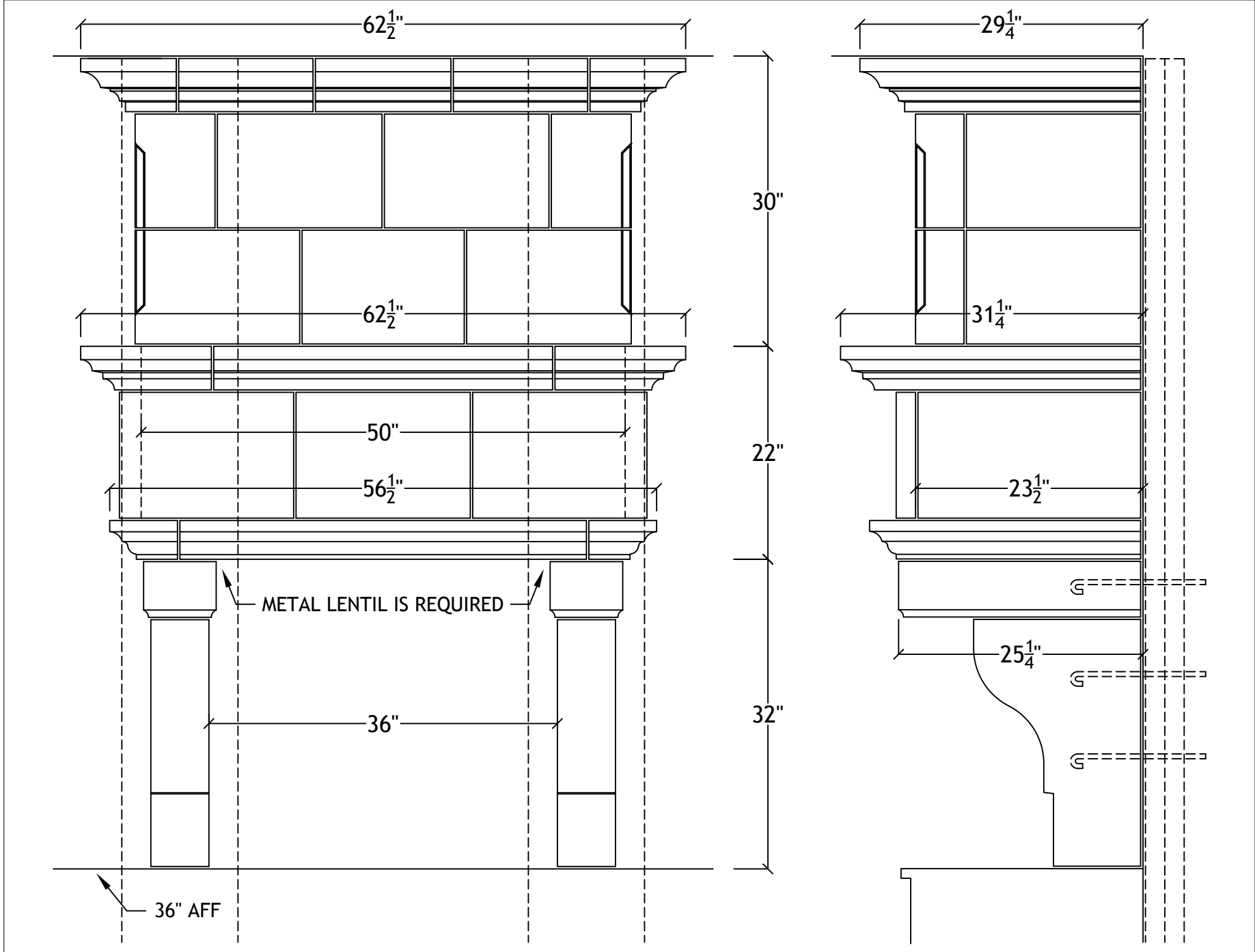
36" Tuscan Range Hood for 10' ceiling
