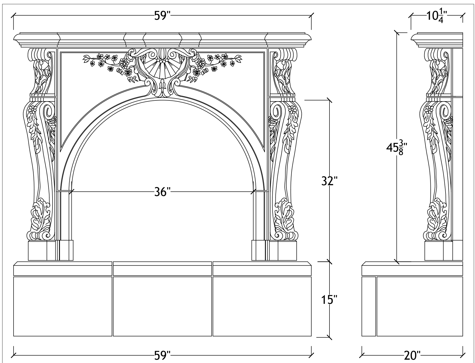
36" Taunton with raised hearth
