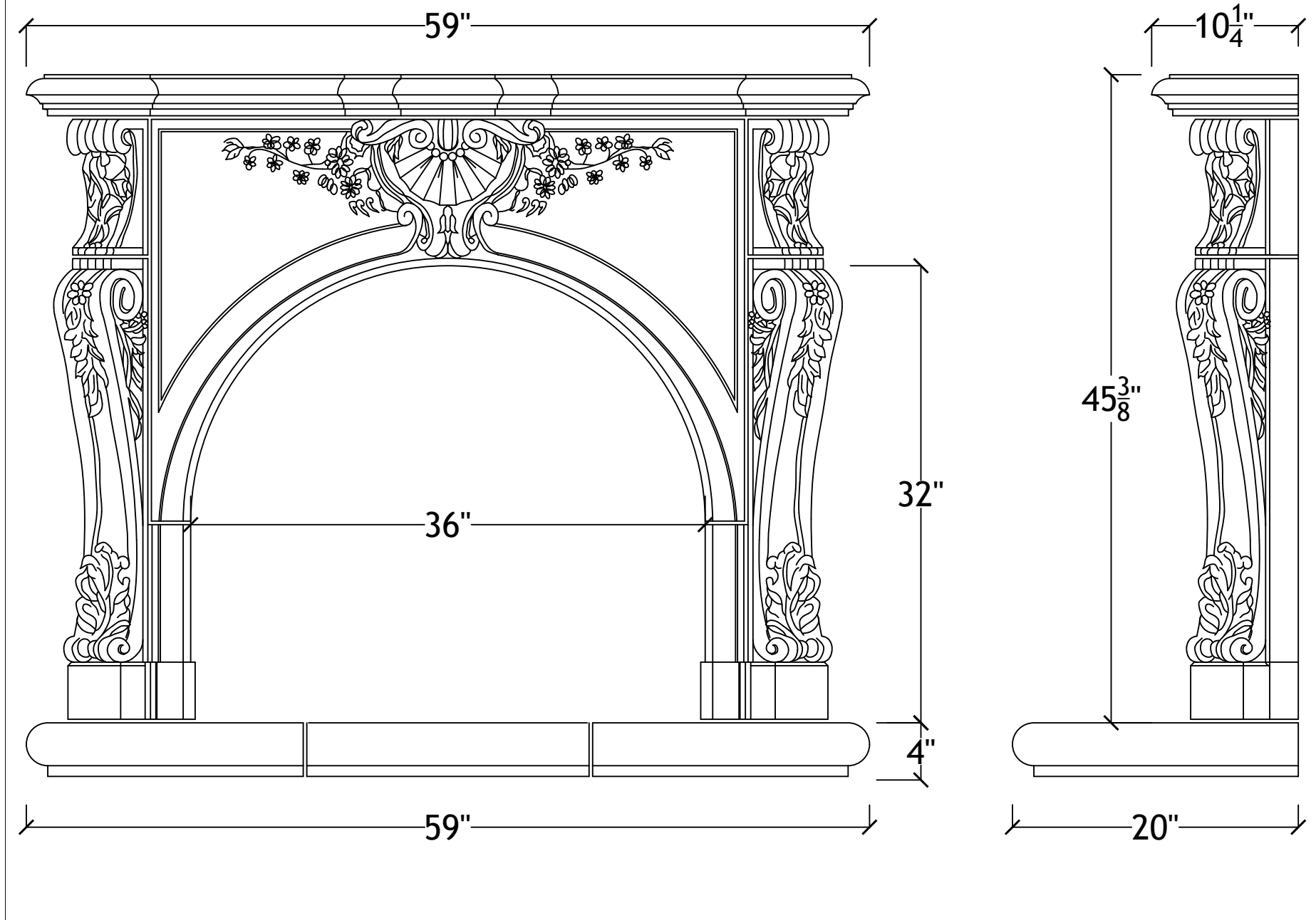
36" Taunton with bullnosed hearth
