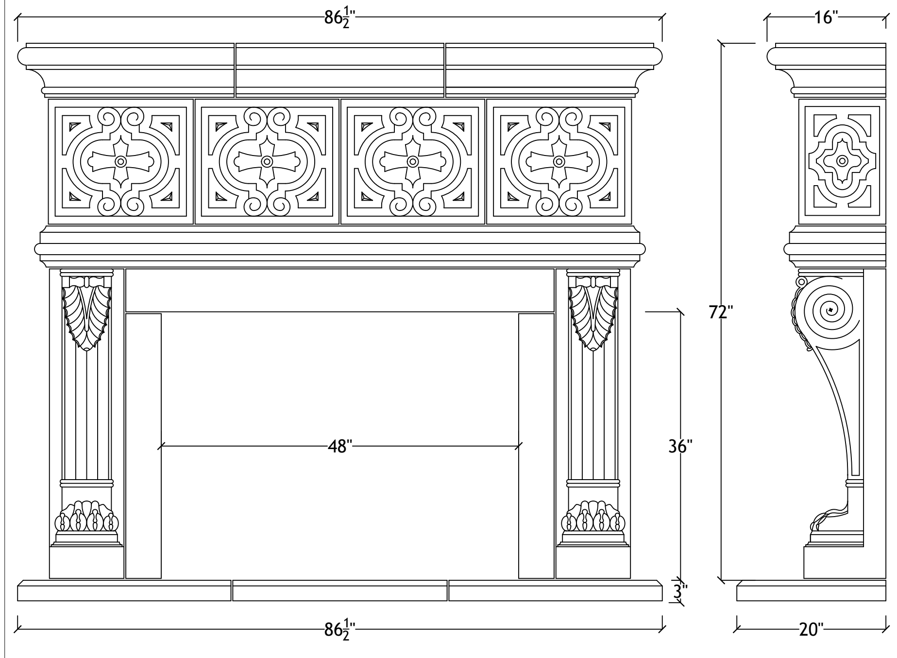
48" Stoneleigh with hearth
