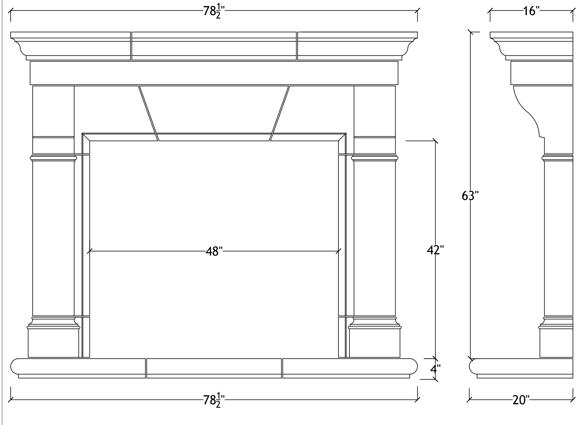
48" Stamford with bullnosed hearth
