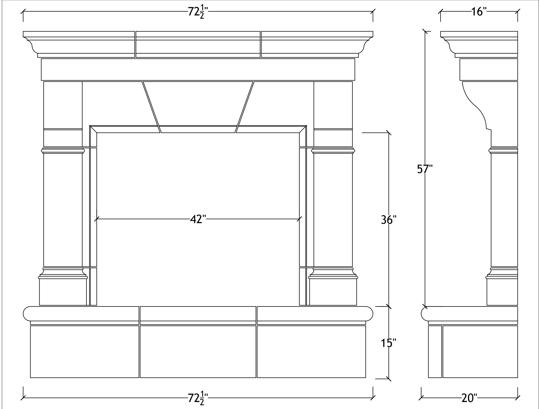
42" Stamford with raised bullnosed hearth
