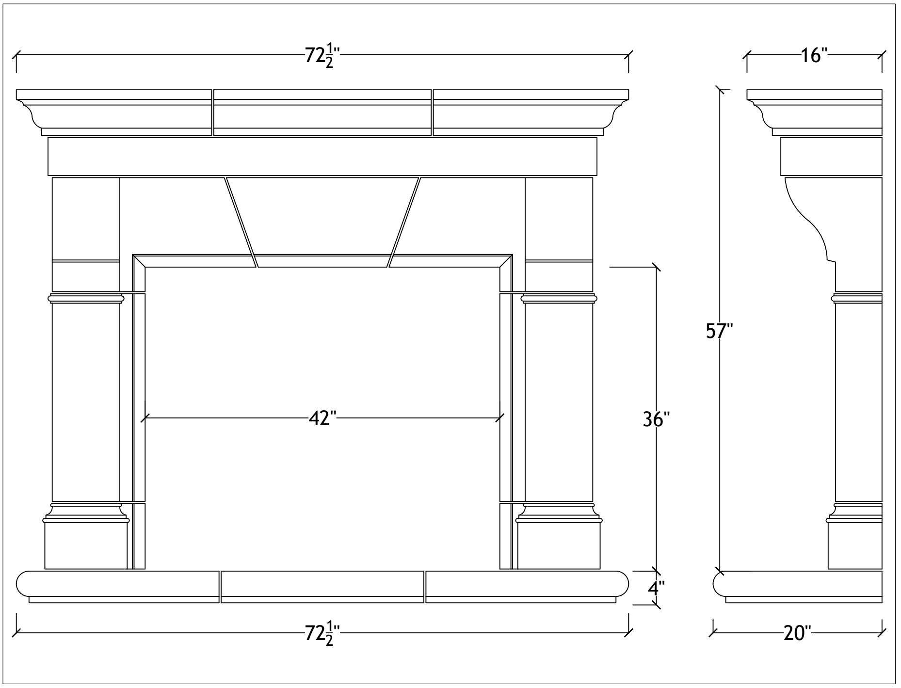
42" Stamford with bullnosed hearth
