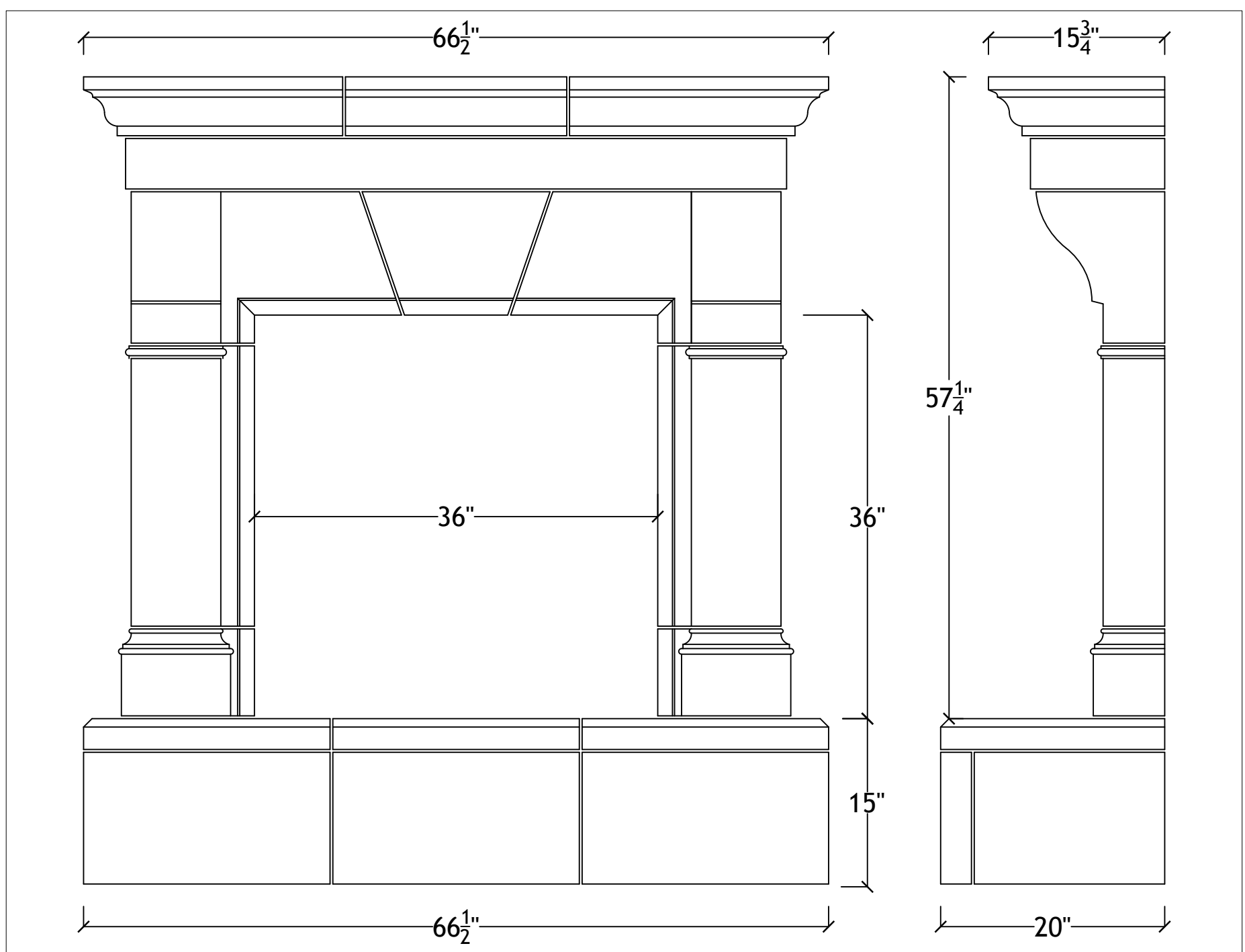
36" Stamford with raised hearth
