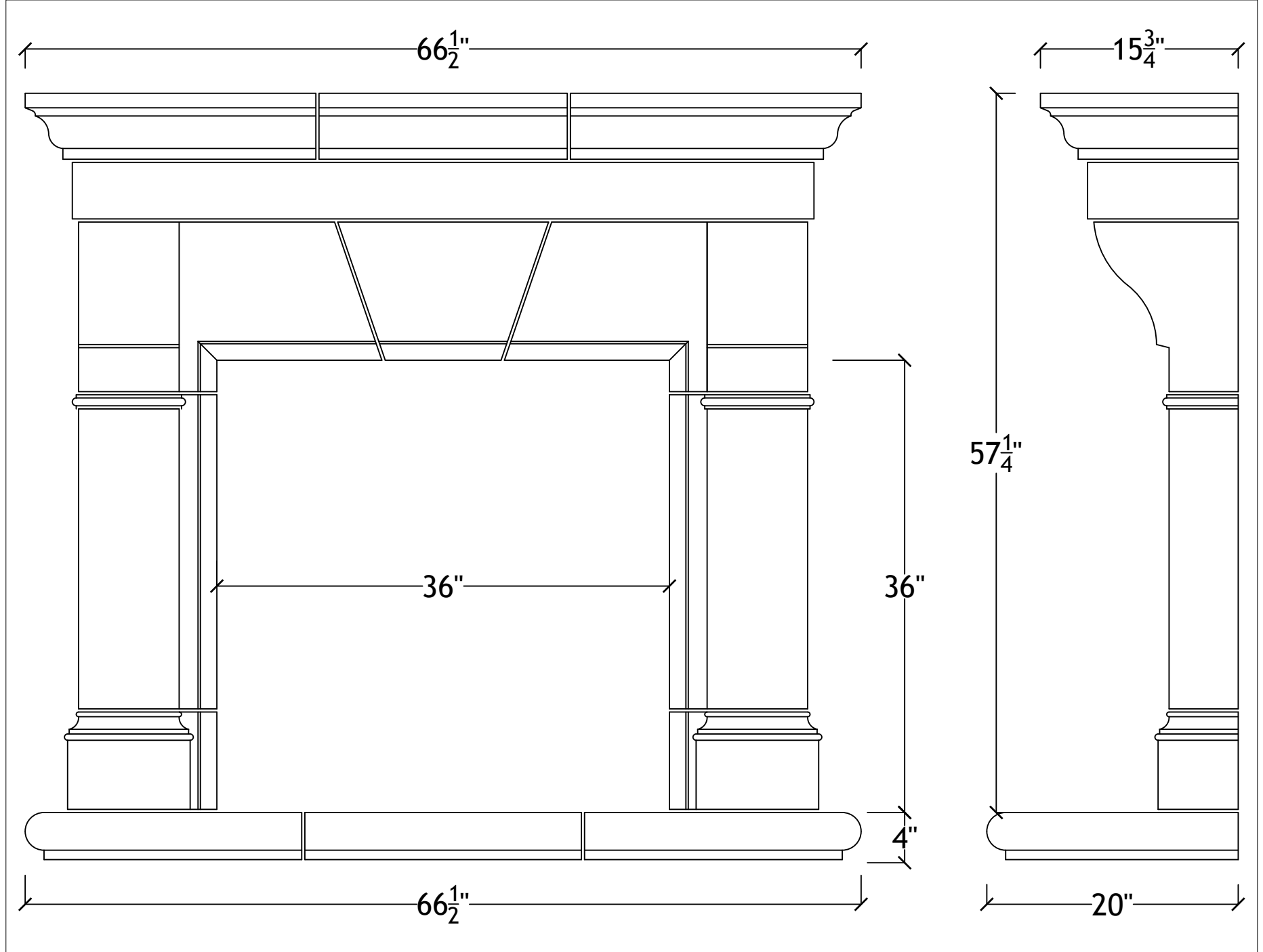
36" Stamford with bullnosed hearth
