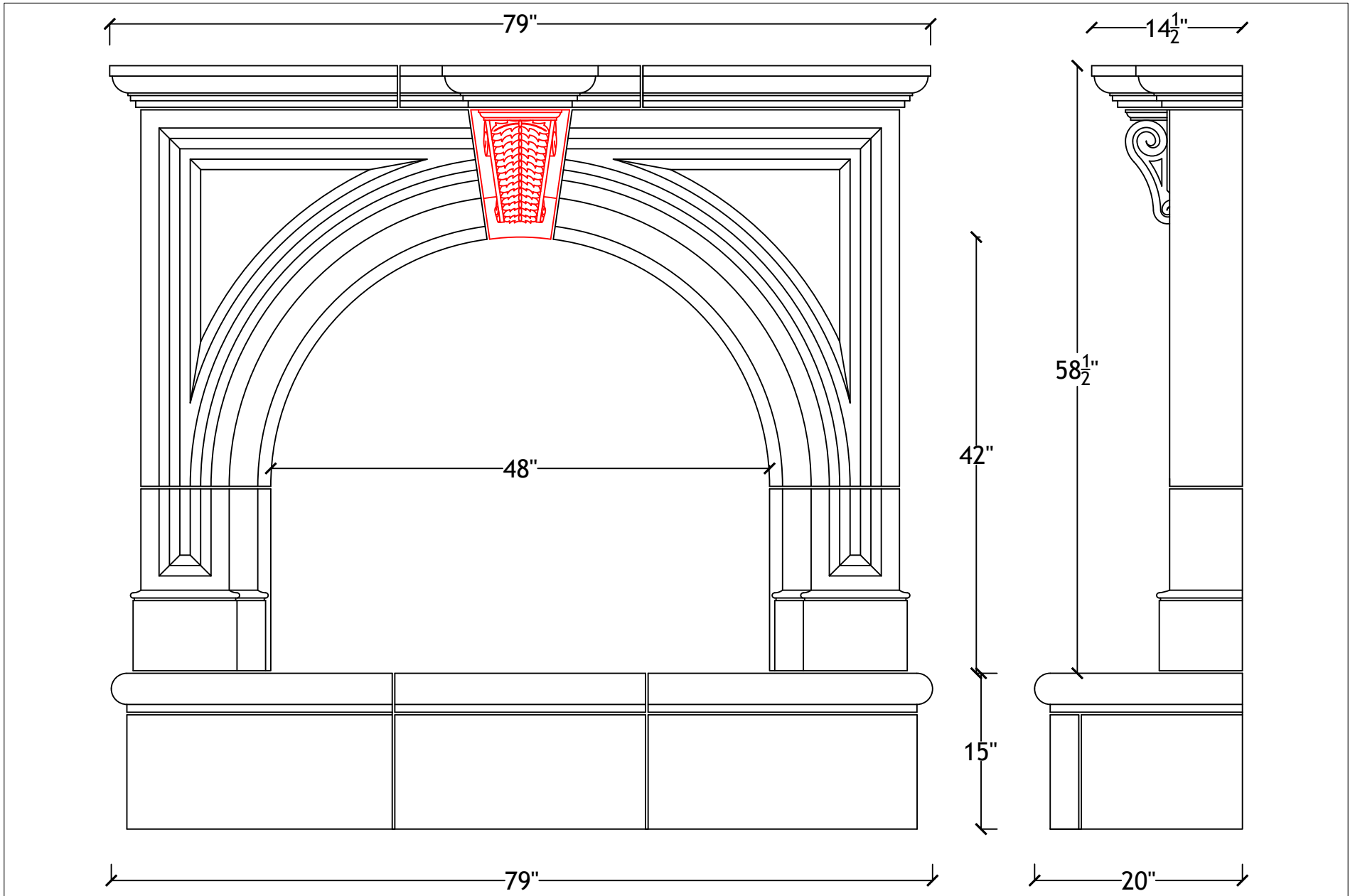
48" Rothton with Raised Bullnose Hearth
