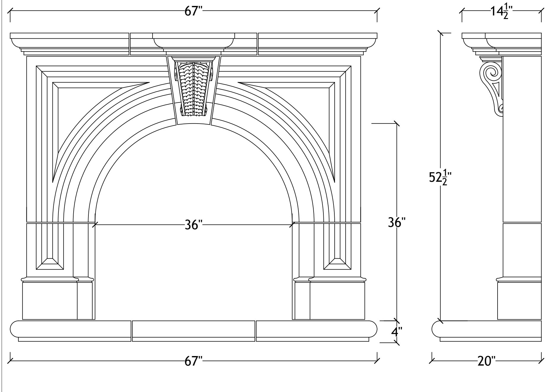
36" Rothton with bullnosed hearth
