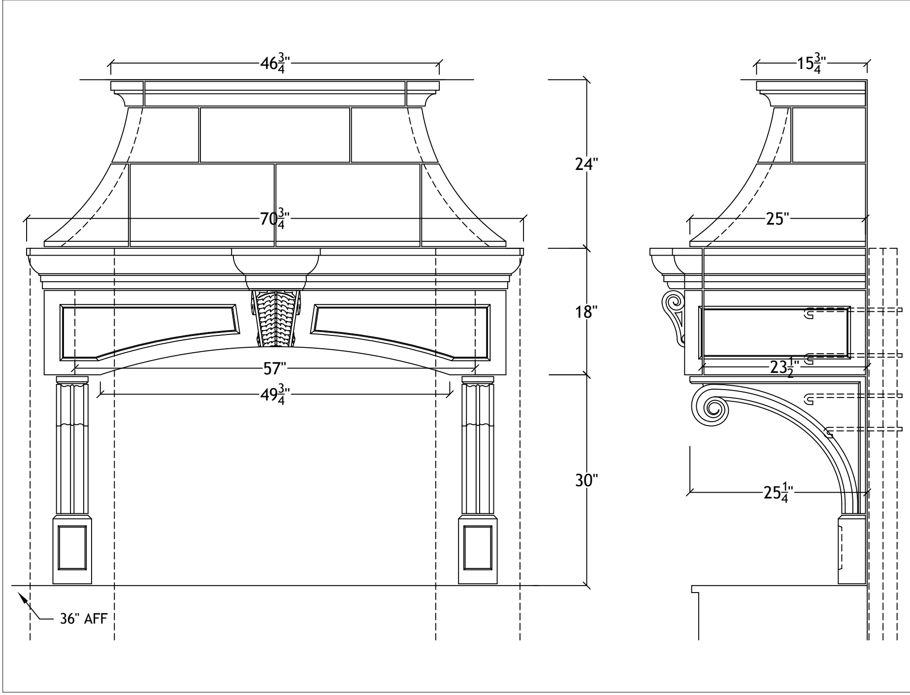
48" Rothchild Range Hood for 9' ceiling
