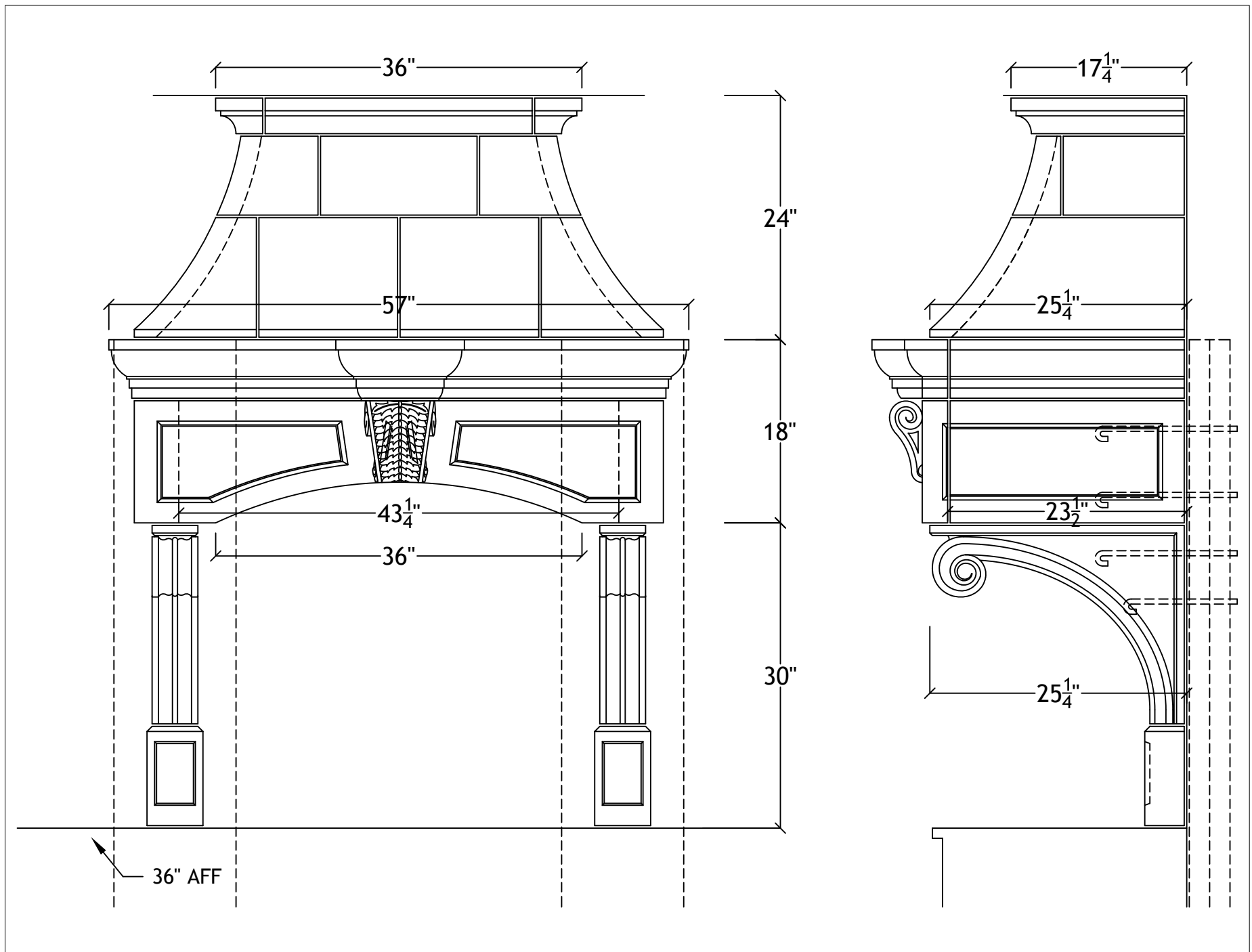
36" Rothchild Range Hood for 9' ceiling
