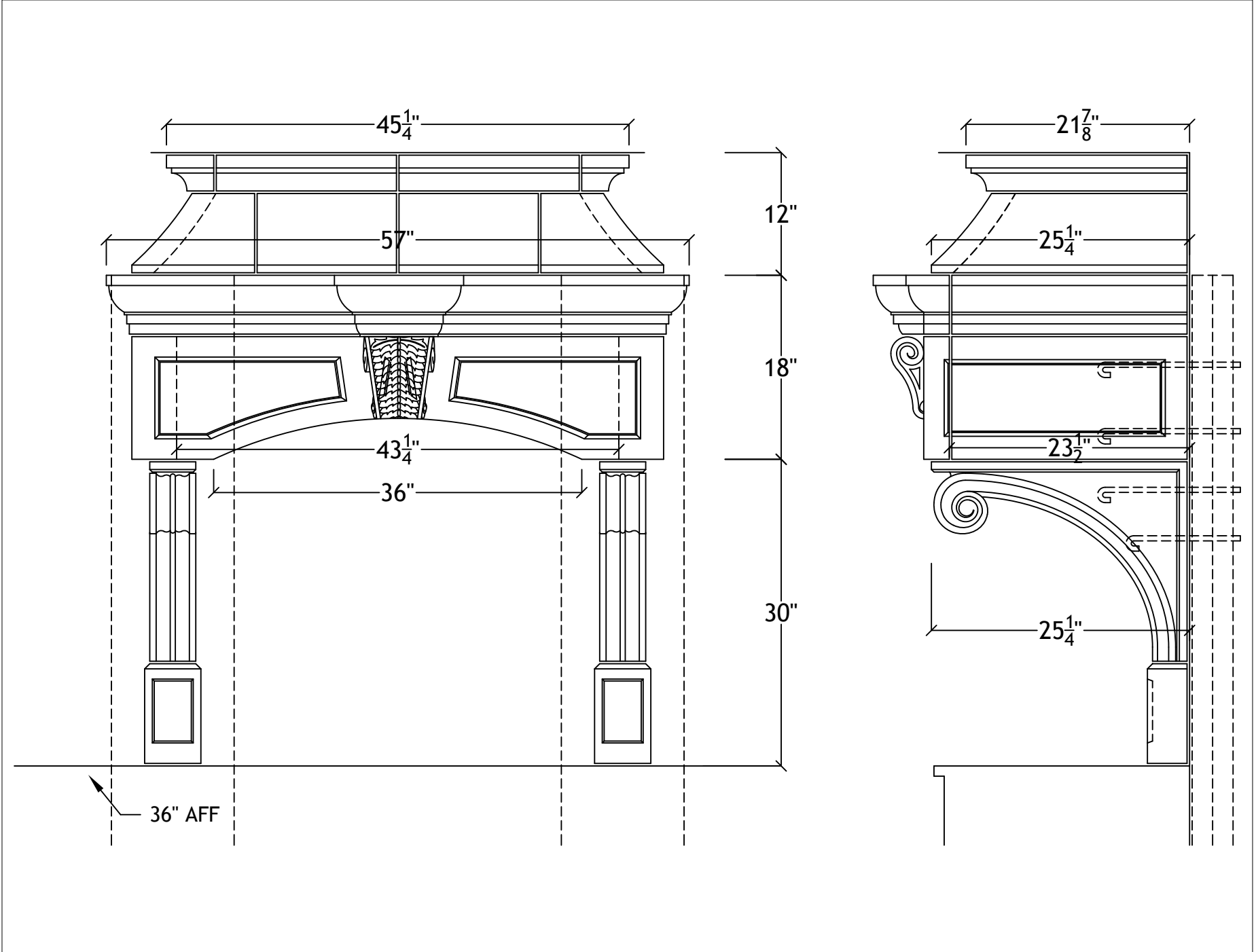
36" Rothchild Range Hood for 8' ceiling
