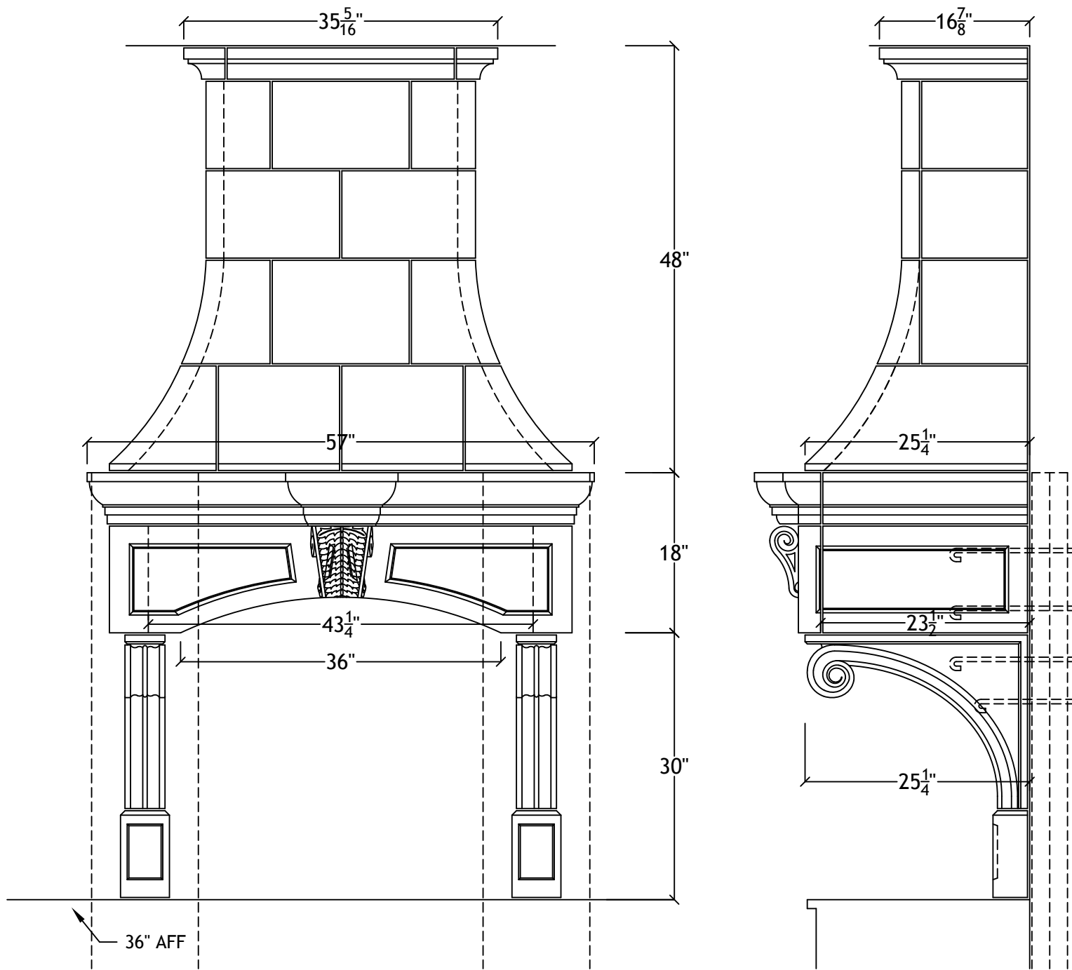
36" Rothchild Range Hood for 11' ceiling
