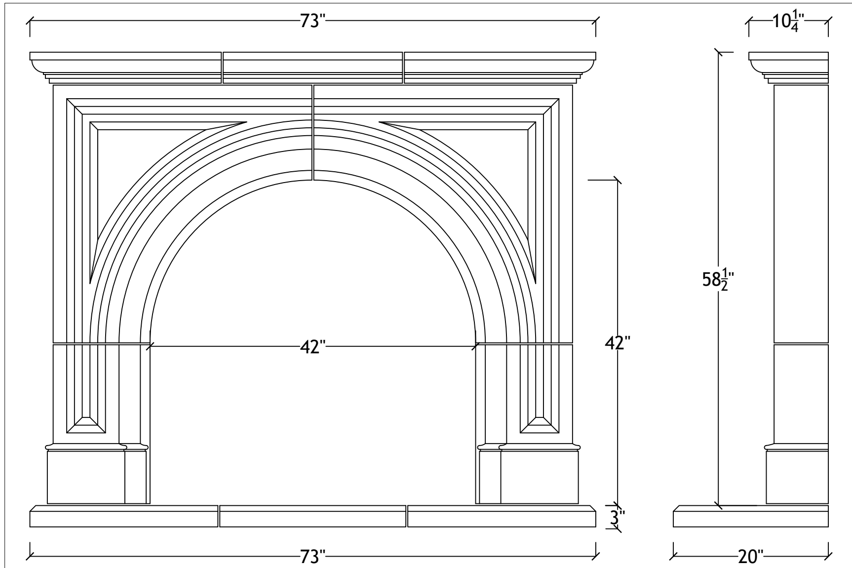
42" Roman with hearth
