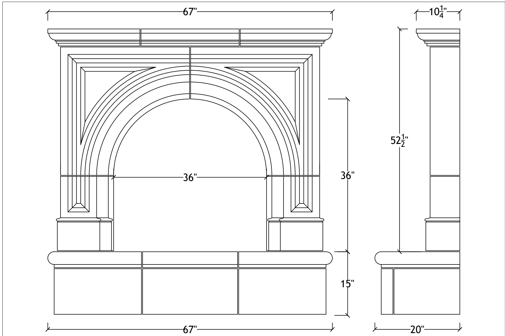
36" Roman with raised bullnosed hearth
