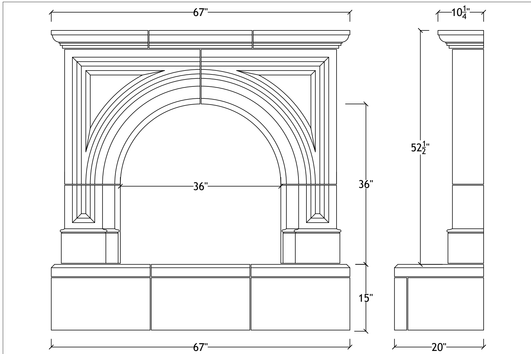
36" Roman with raised hearth
