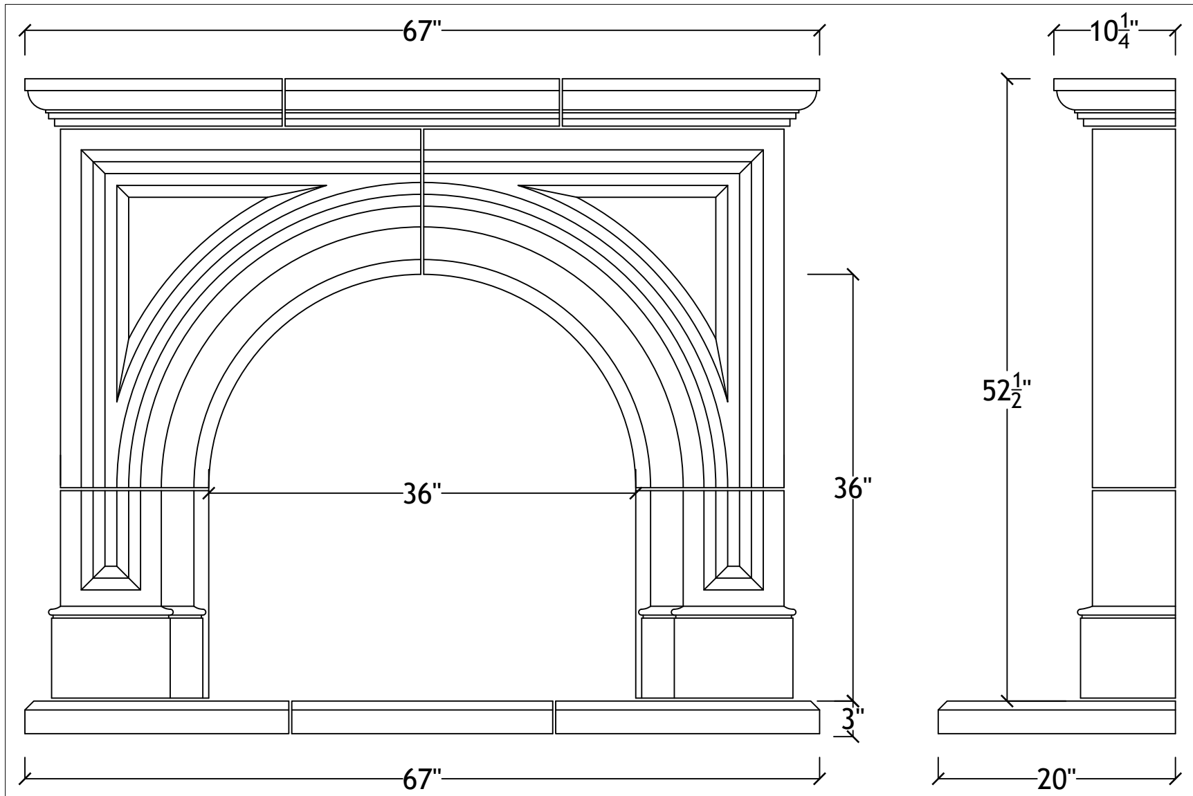
36" Roman with hearth
