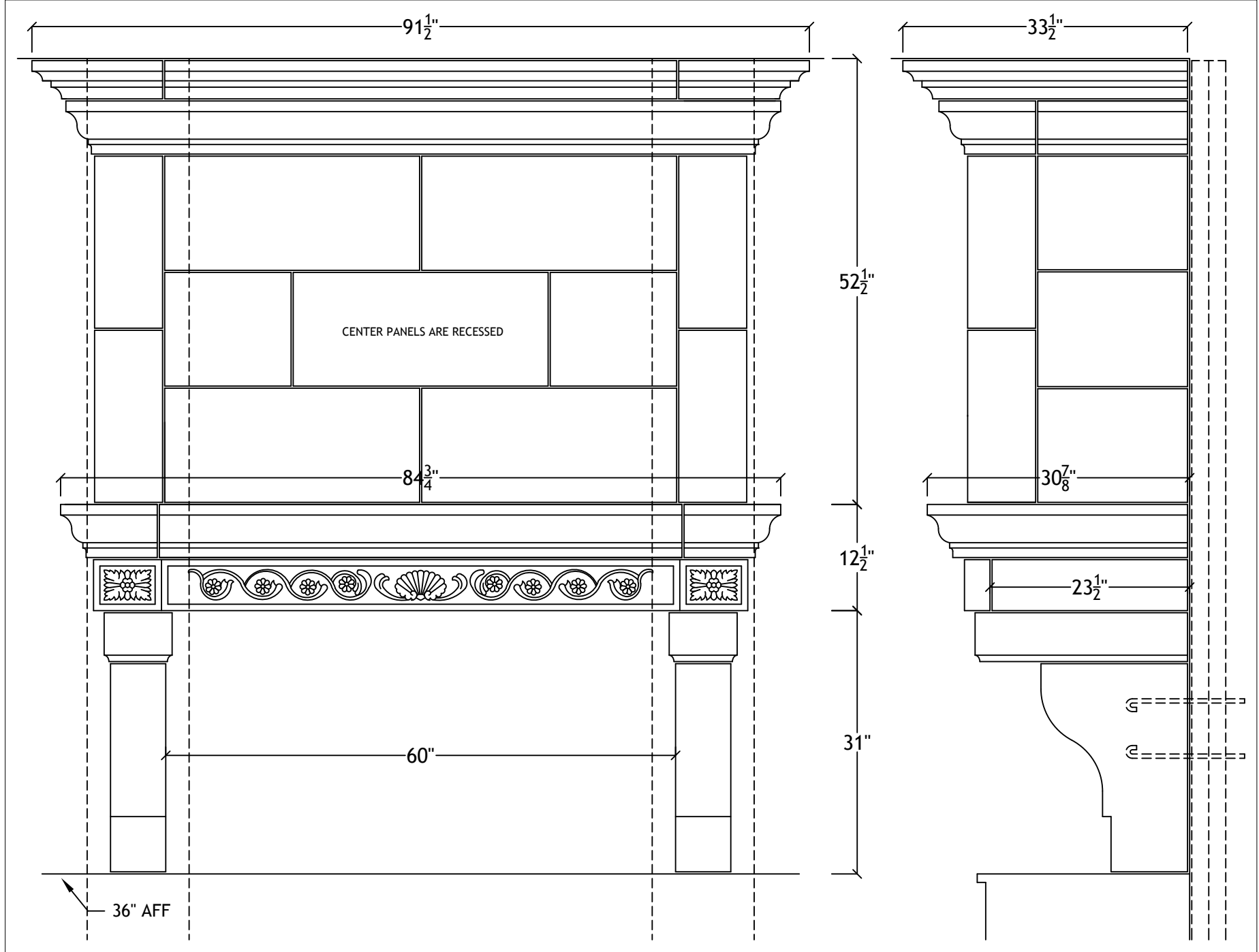
60" Rhapsody Range Hood for 10' ceiling
