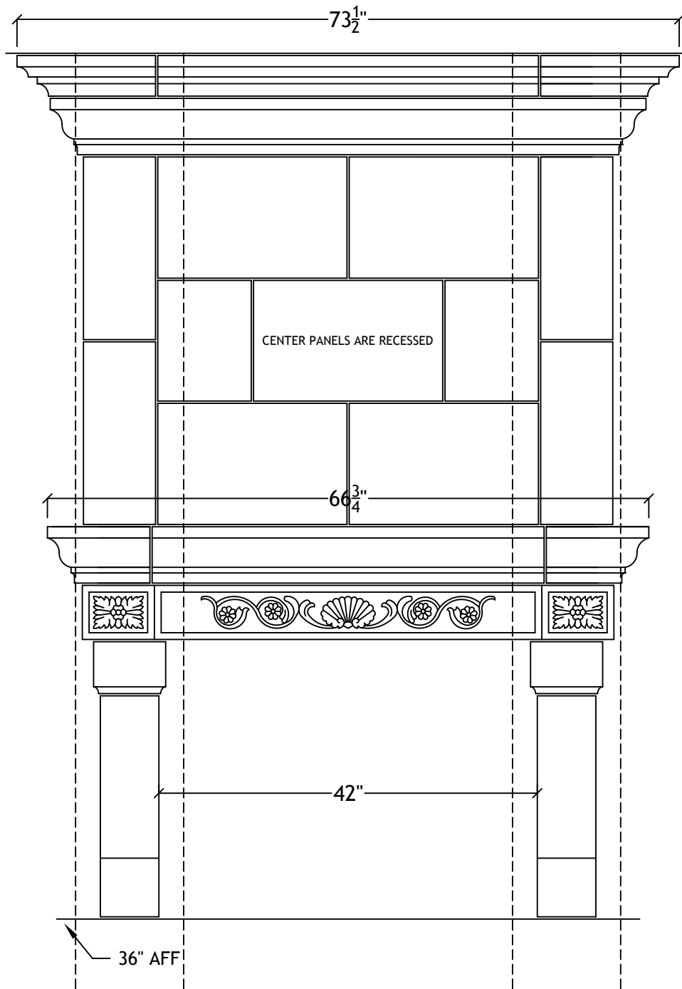
42" Rhapsody Range Hood for 11' ceiling
