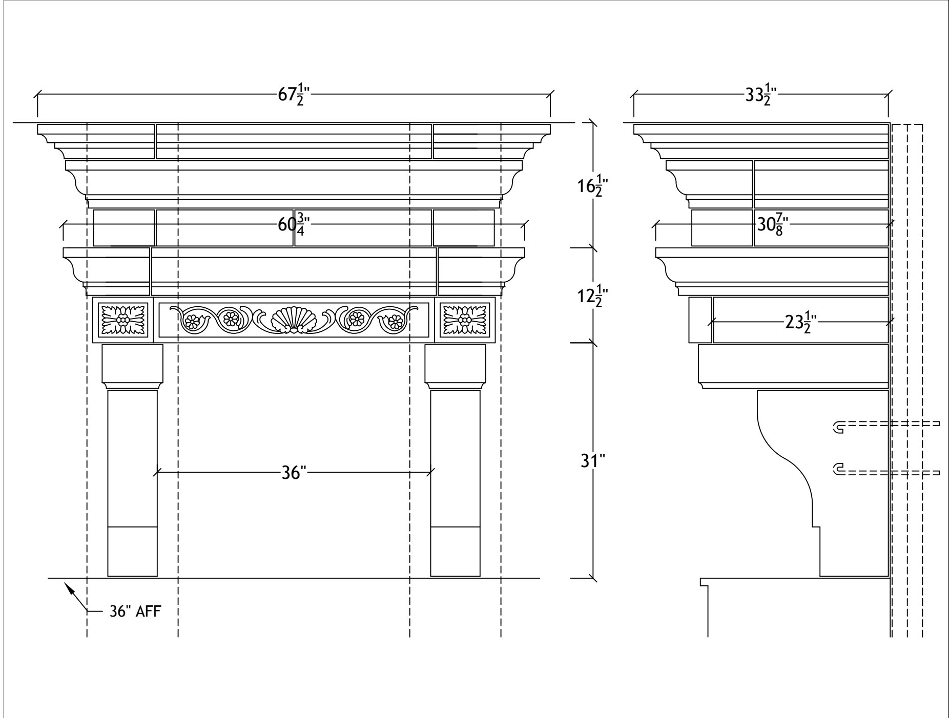
36" Rhapsody Range Hood for 8' ceiling
