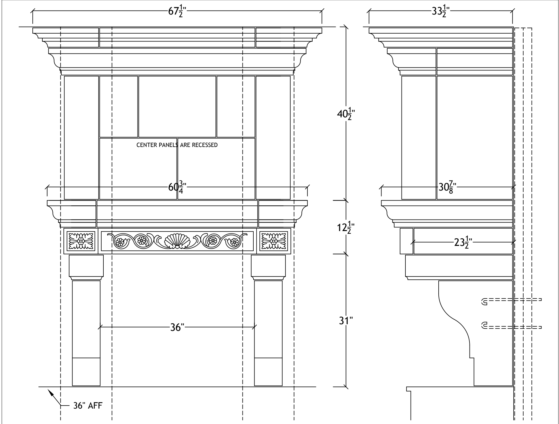
36" Rhapsody Range Hood for 10' ceiling
