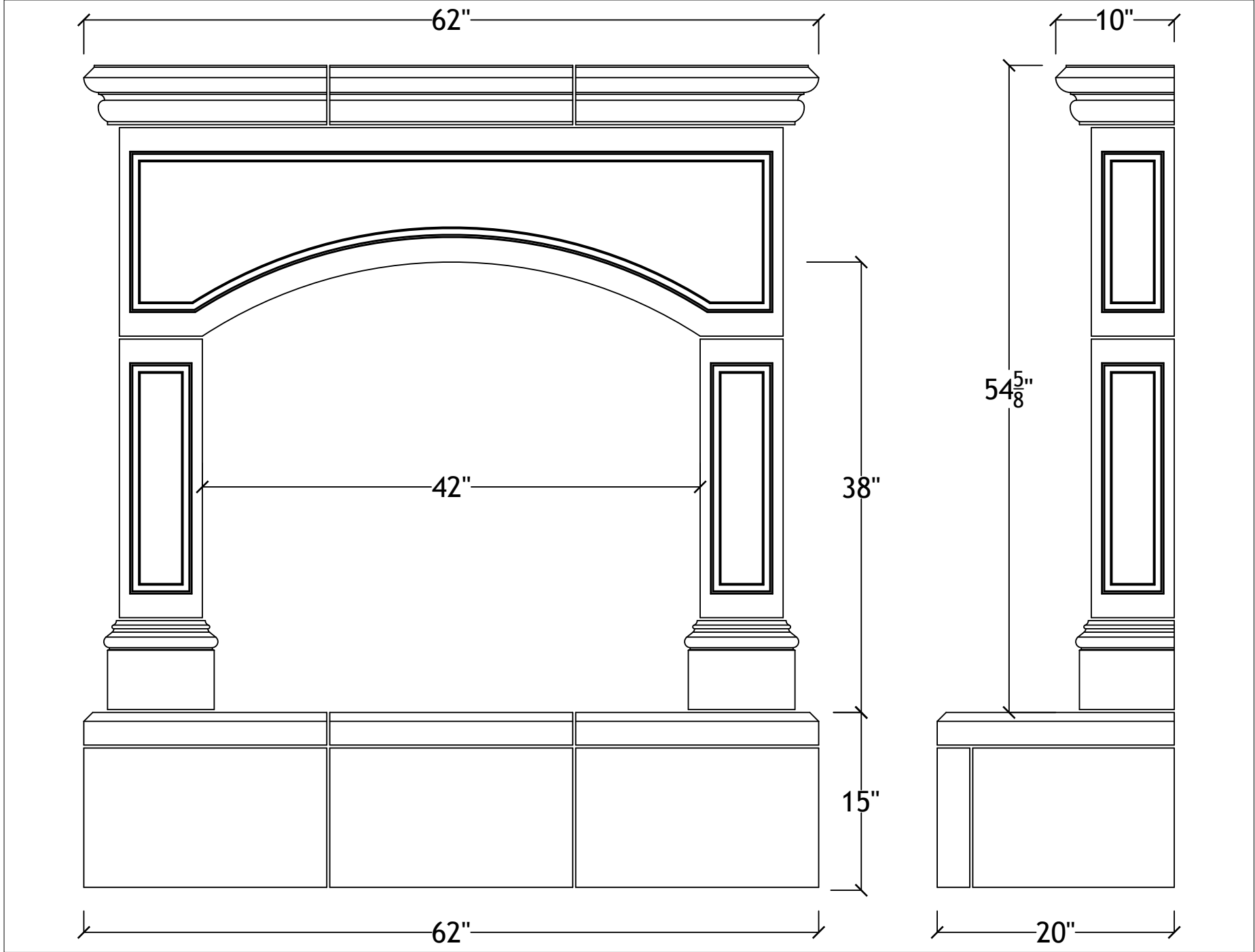
42" Oxford with raised hearth
