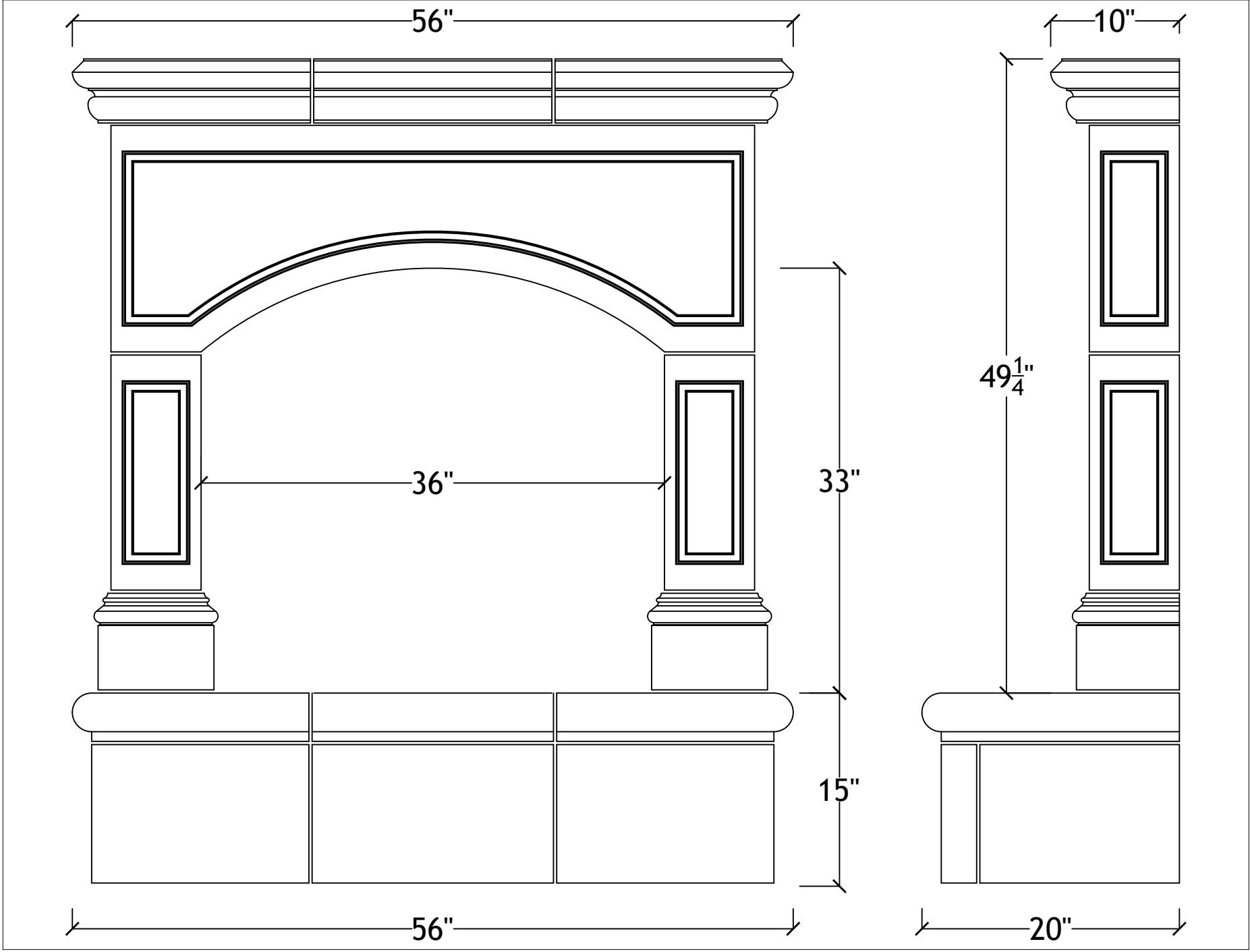
36" Oxford with raised bullnosed hearth
