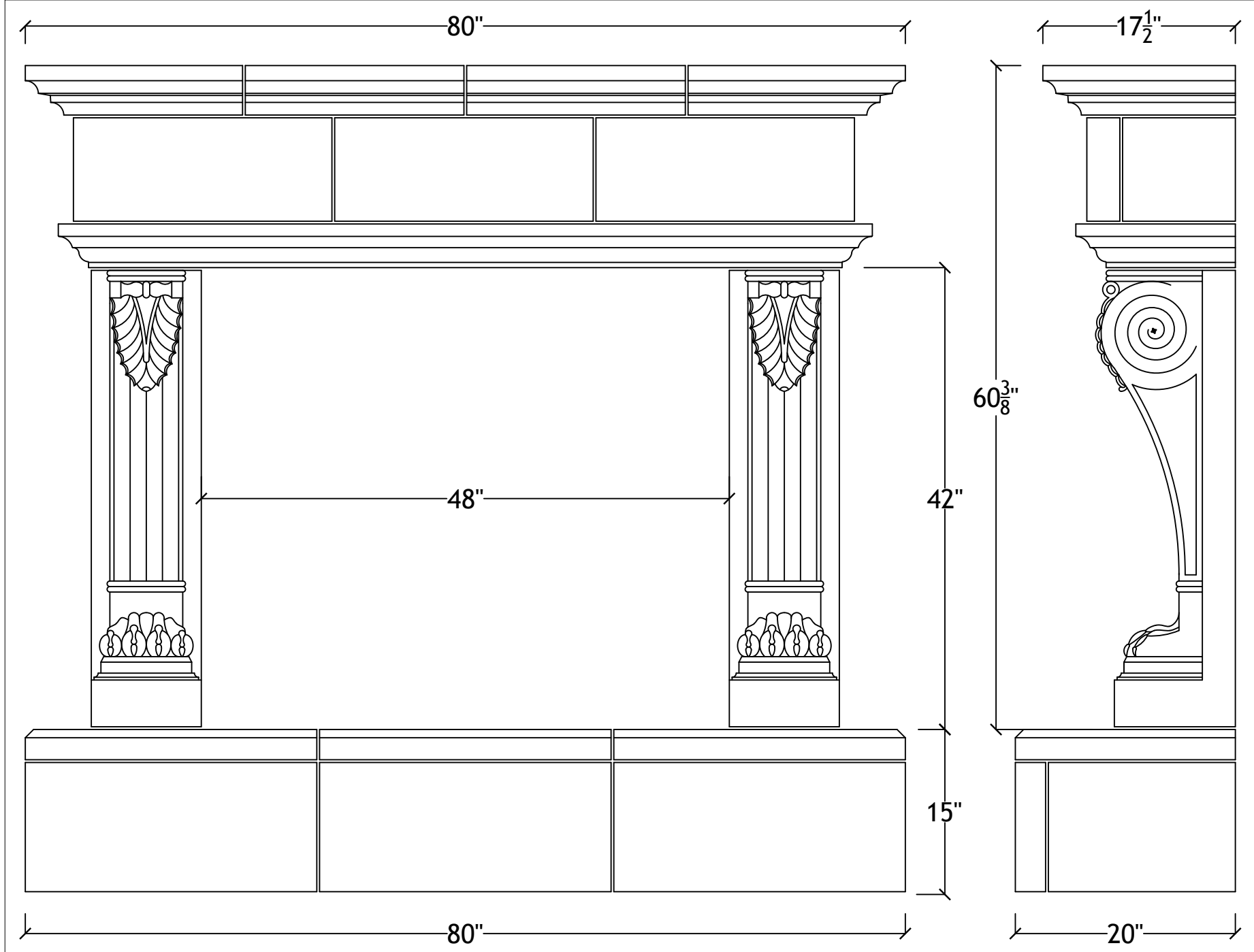
48" Nottingham with raised hearth
