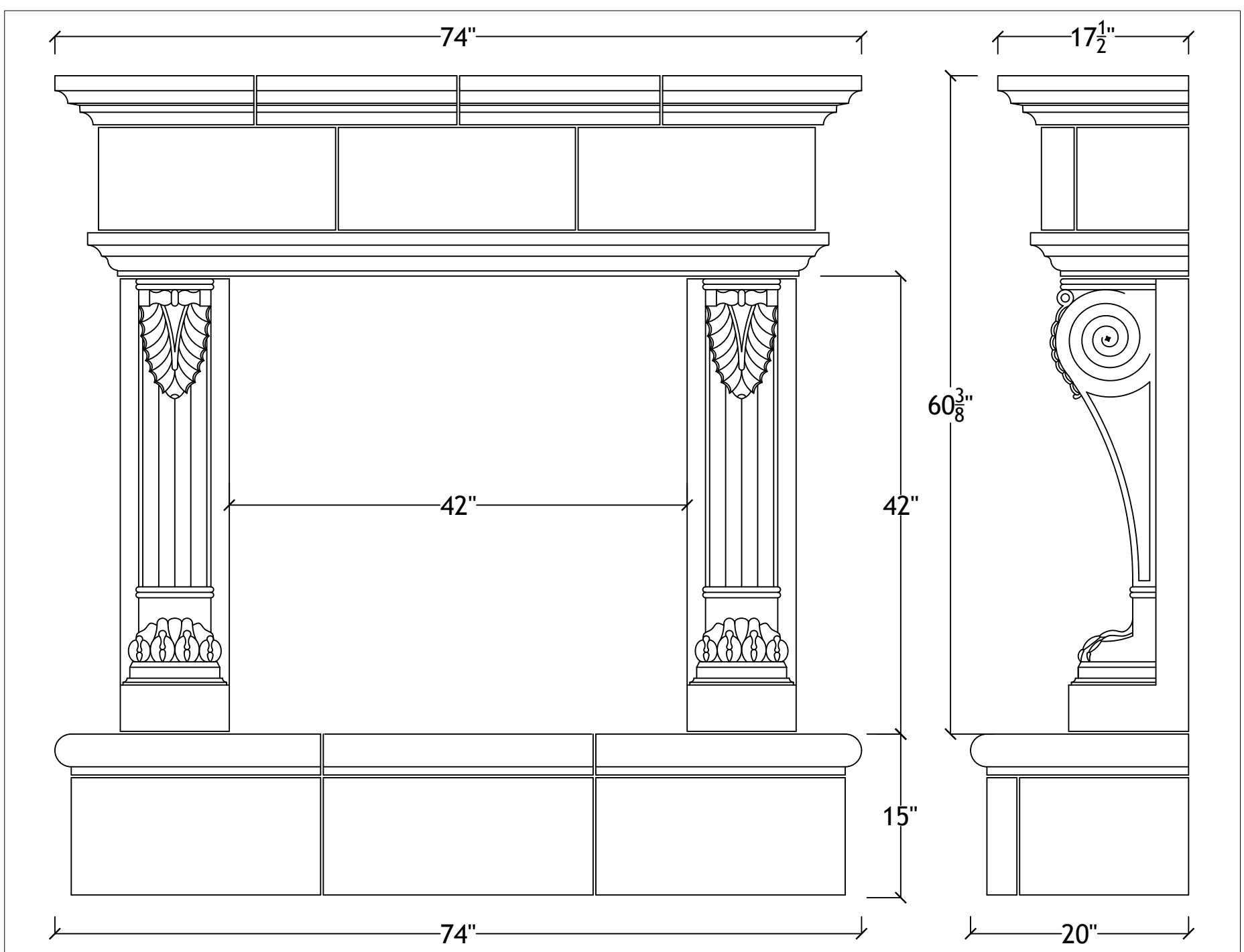
42" Nottingham with raised bullnosed hearth
