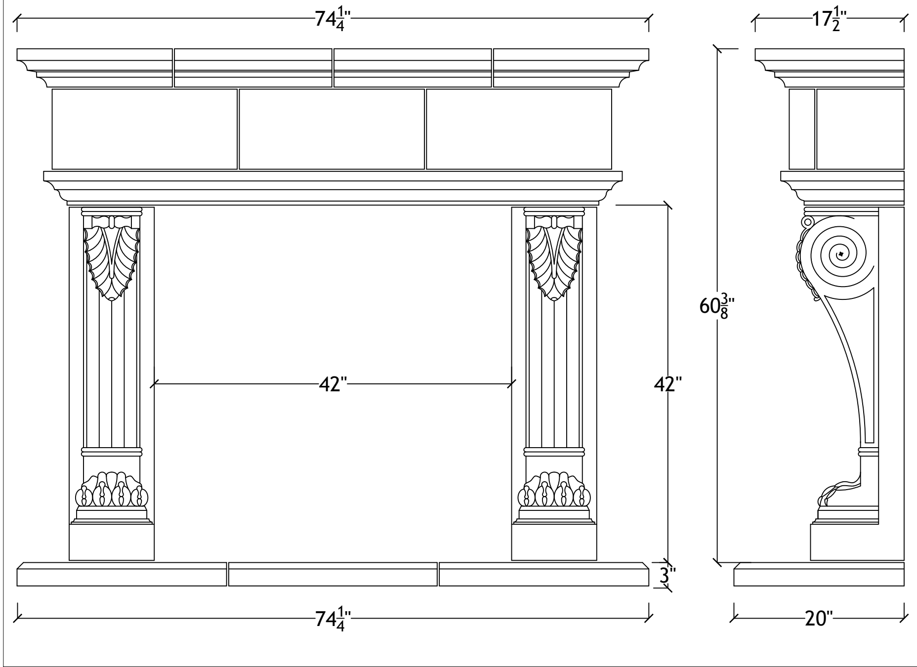
42" Nottingham with hearth
